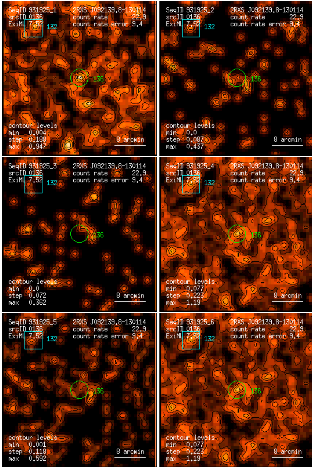
Figure 136: RASS 931925: detection 0136: band rate images, Gaussian filter: (1) PSPC channels 11 – 41, (2) 52 – 90, (3) 91 – 201, (4) 11 – 235, (5) 52 – 201, (6) 11 – 201. Broad band rates in counts/ks. Band rate contour levels in counts/ks/arcmin 2 .
