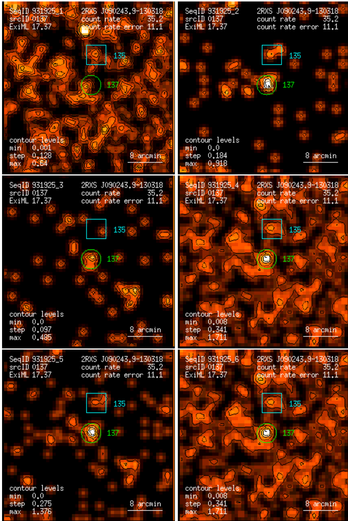
Figure 137: RASS 931925: detection 0137: band rate images, Gaussian filter: (1) PSPC channels 11 – 41, (2) 52 – 90, (3) 91 – 201, (4) 11 – 235, (5) 52 – 201, (6) 11 – 201. Broad band rates in counts/ks. Band rate contour levels in counts/ks/arcmin 2 .
