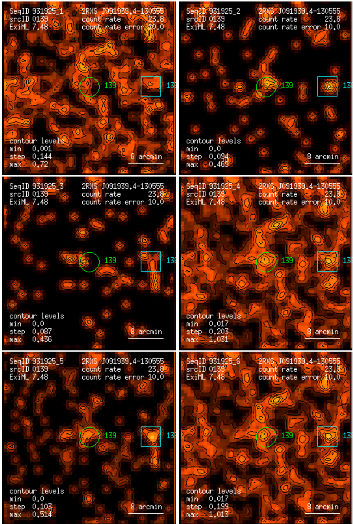
Figure 139: RASS 931925: detection 0139: band rate images, Gaussian filter: (1) PSPC channels 11 – 41, (2) 52 – 90, (3) 91 – 201, (4) 11 – 235, (5) 52 – 201, (6) 11 – 201. Broad band rates in counts/ks. Band rate contour levels in counts/ks/arcmin 2 .
