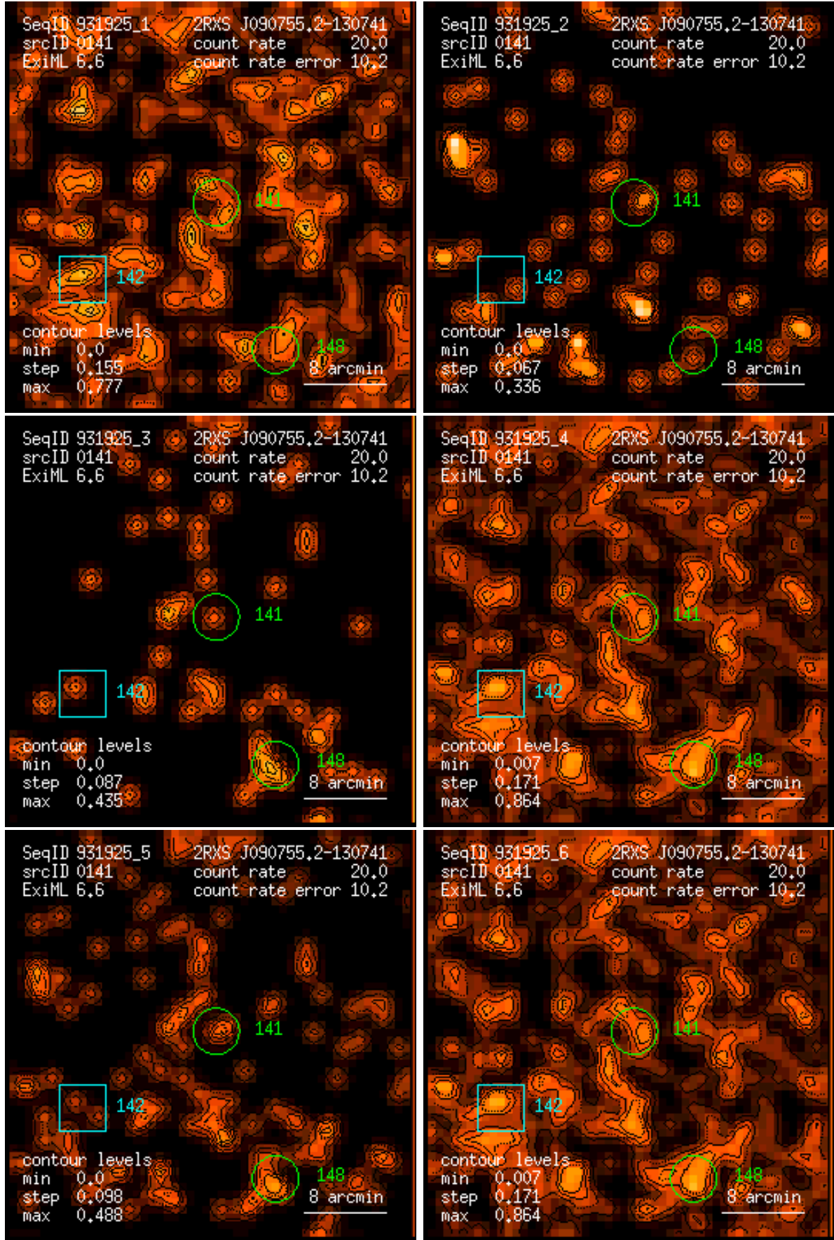
Figure 141: RASS 931925: detection 0141: band rate images, Gaussian filter: (1) PSPC channels 11 – 41, (2) 52 – 90, (3) 91 – 201, (4) 11 – 235, (5) 52 – 201, (6) 11 – 201. Broad band rates in counts/ks. Band rate contour levels in counts/ks/arcmin 2 .
