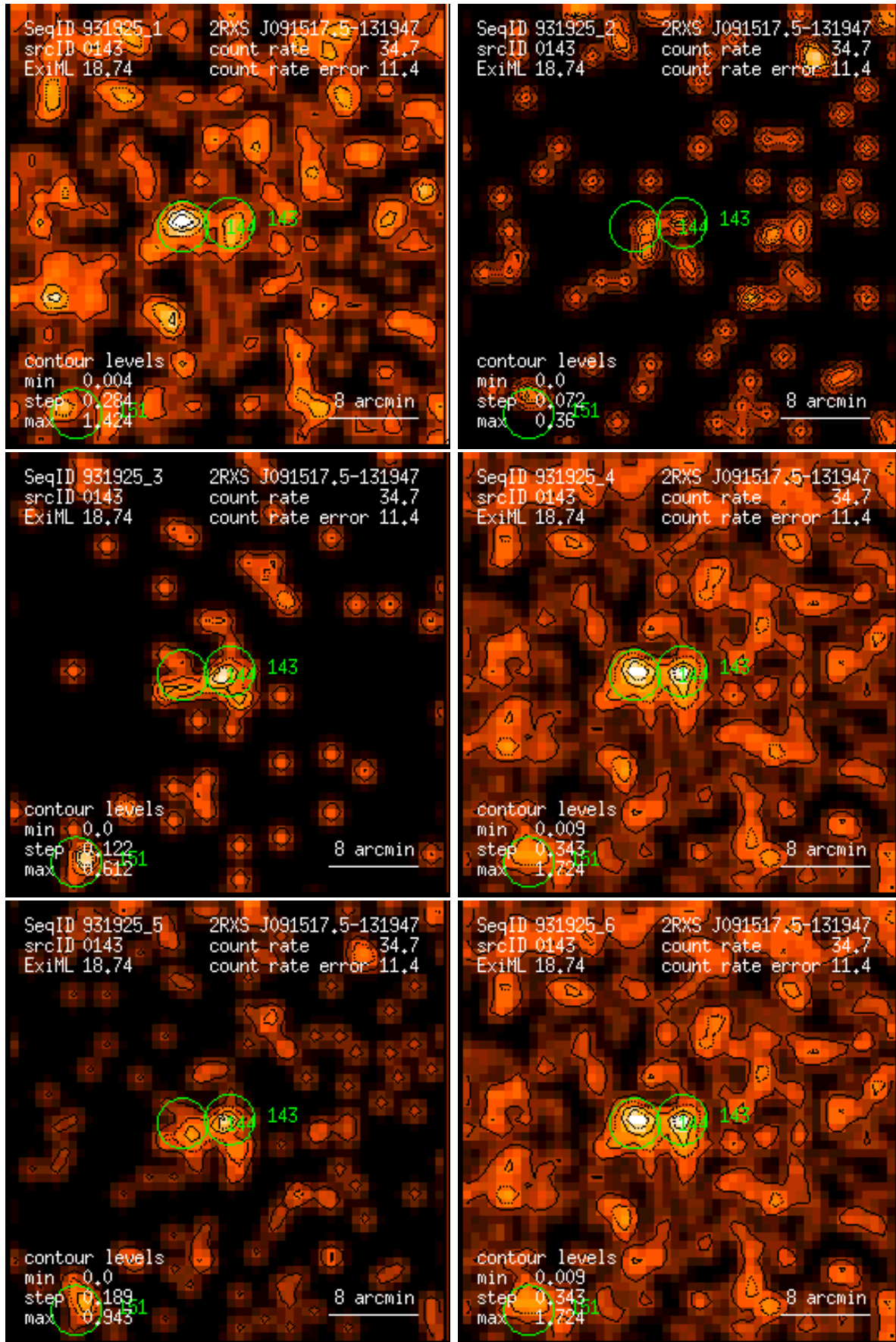
Figure 143: RASS 931925: detection 0143: band rate images, Gaussian filter: (1) PSPC channels 11 – 41, (2) 52 – 90, (3) 91 – 201, (4) 11 – 235, (5) 52 – 201, (6) 11 – 201. Broad band rates in counts/ks. Band rate contour levels in counts/ks/arcmin 2 .
