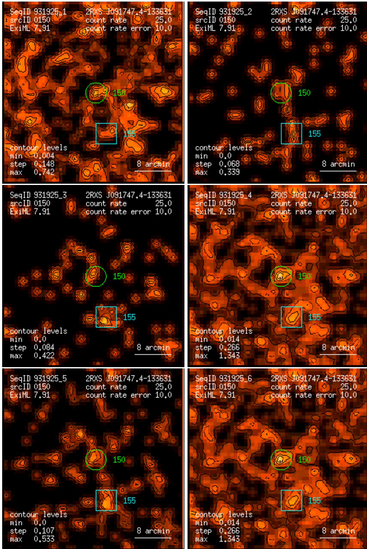
Figure 150: RASS 931925: detection 0150: band rate images, Gaussian filter: (1) PSPC channels 11 – 41, (2) 52 – 90, (3) 91 – 201, (4) 11 – 235, (5) 52 – 201, (6) 11 – 201. Broad band rates in counts/ks. Band rate contour levels in counts/ks/arcmin 2 .
