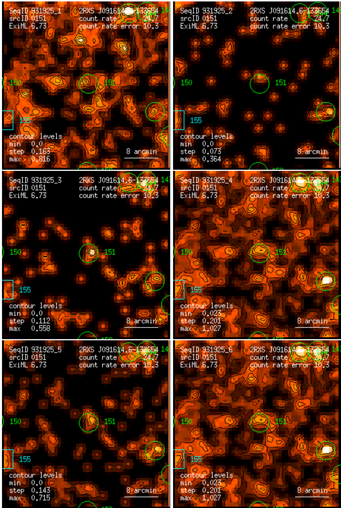
Figure 151: RASS 931925: detection 0151: band rate images, Gaussian filter: (1) PSPC channels 11 – 41, (2) 52 – 90, (3) 91 – 201, (4) 11 – 235, (5) 52 – 201, (6) 11 – 201. Broad band rates in counts/ks. Band rate contour levels in counts/ks/arcmin 2 .
