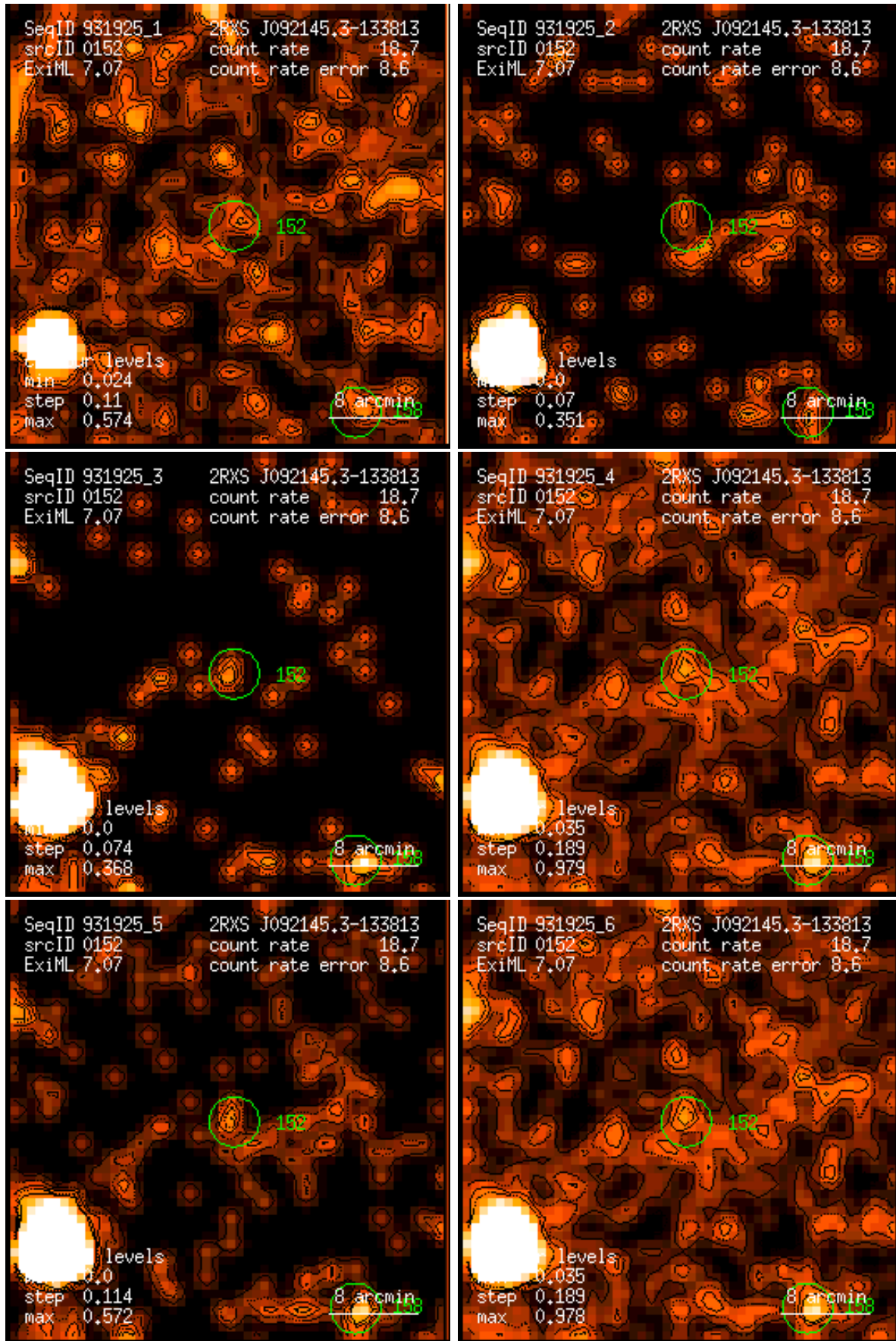
Figure 152: RASS 931925: detection 0152: band rate images, Gaussian filter: (1) PSPC channels 11 – 41, (2) 52 – 90, (3) 91 – 201, (4) 11 – 235, (5) 52 – 201, (6) 11 – 201. Broad band rates in counts/ks. Band rate contour levels in counts/ks/arcmin 2 .
