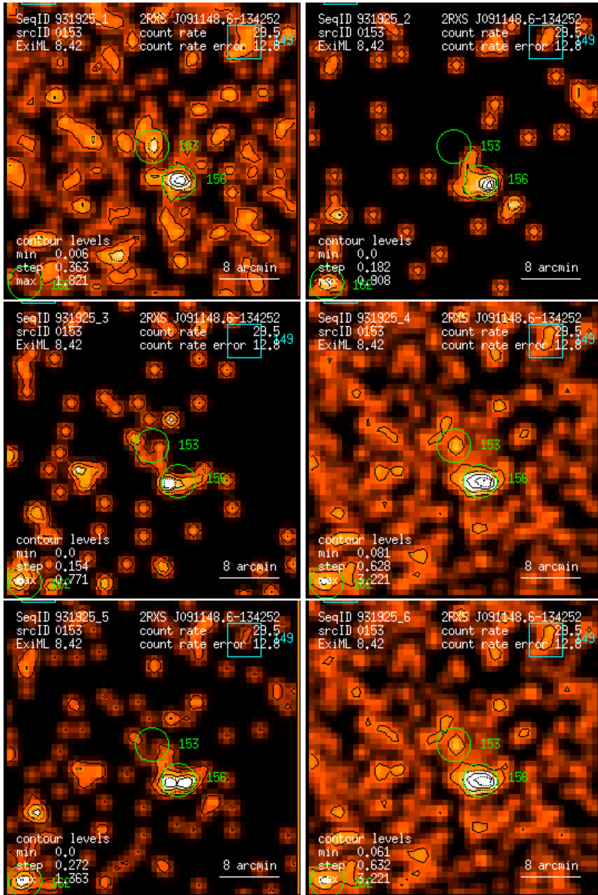
Figure 153: RASS 931925: detection 0153: band rate images, Gaussian filter: (1) PSPC channels 11 – 41, (2) 52 – 90, (3) 91 – 201, (4) 11 – 235, (5) 52 – 201, (6) 11 – 201. Broad band rates in counts/ks. Band rate contour levels in counts/ks/arcmin 2 .
