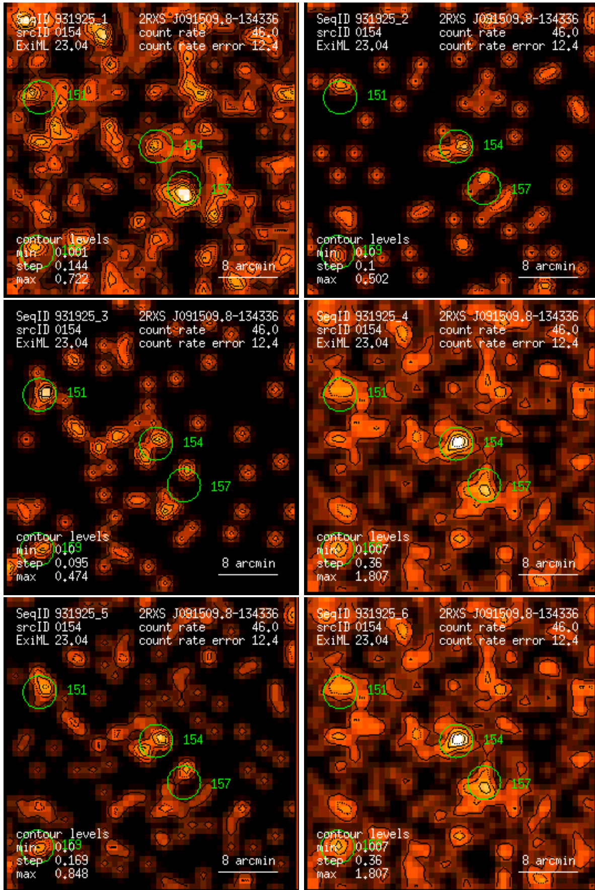
Figure 154: RASS 931925: detection 0154: band rate images, Gaussian filter: (1) PSPC channels 11 – 41, (2) 52 – 90, (3) 91 – 201, (4) 11 – 235, (5) 52 – 201, (6) 11 – 201. Broad band rates in counts/ks. Band rate contour levels in counts/ks/arcmin 2 .
