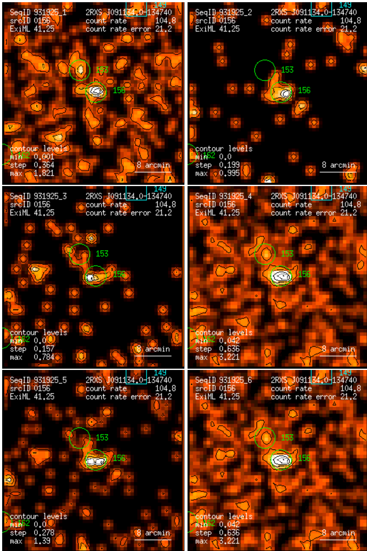
Figure 156: RASS 931925: detection 0156: band rate images, Gaussian filter: (1) PSPC channels 11 – 41, (2) 52 – 90, (3) 91 – 201, (4) 11 – 235, (5) 52 – 201, (6) 11 – 201. Broad band rates in counts/ks. Band rate contour levels in counts/ks/arcmin 2 .
