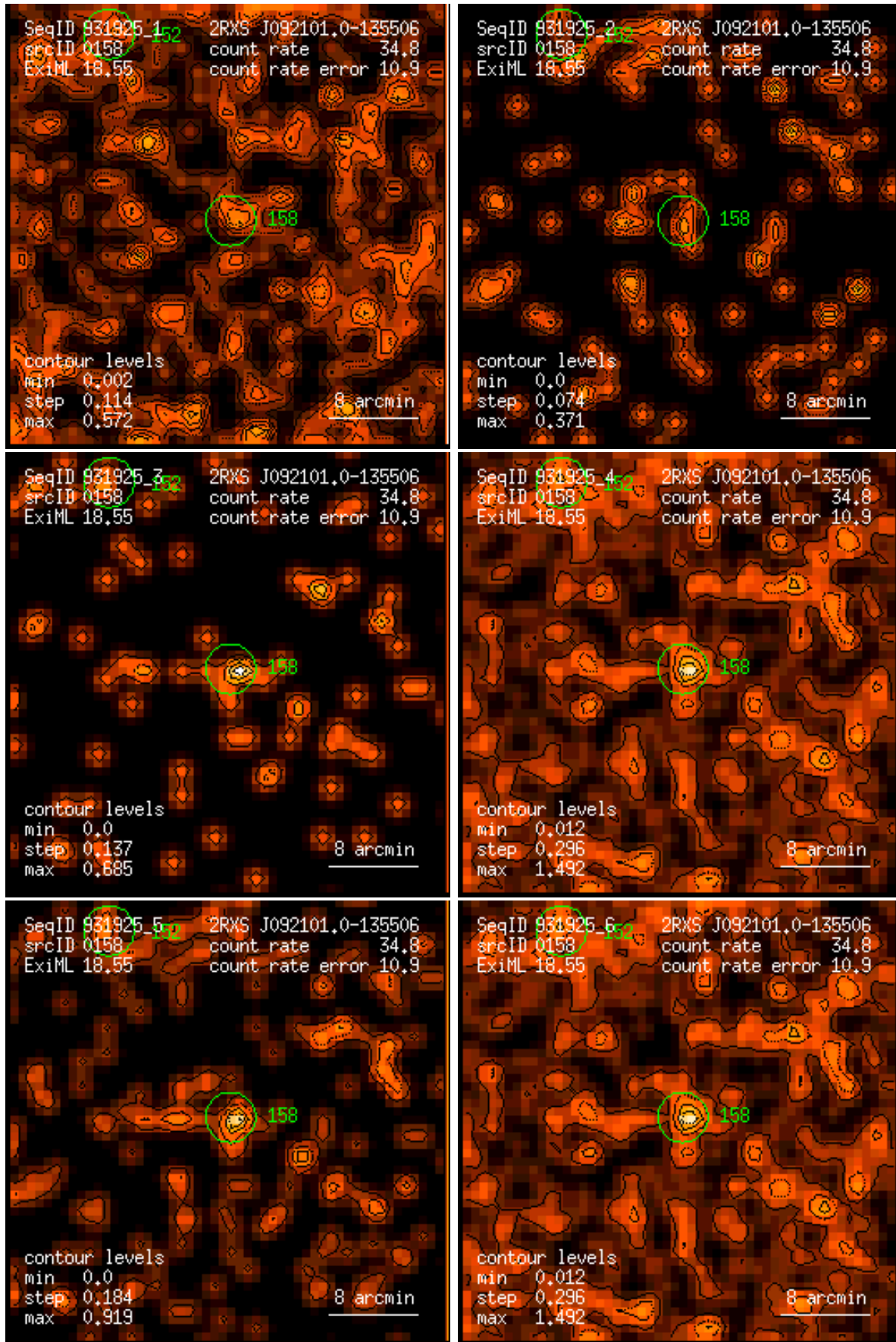
Figure 158: RASS 931925: detection 0158: band rate images, Gaussian filter: (1) PSPC channels 11 – 41, (2) 52 – 90, (3) 91 – 201, (4) 11 – 235, (5) 52 – 201, (6) 11 – 201. Broad band rates in counts/ks. Band rate contour levels in counts/ks/arcmin 2 .
