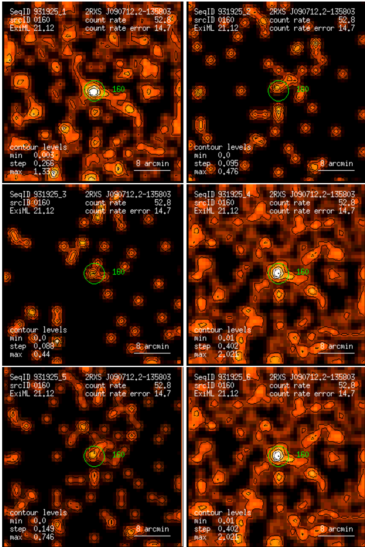
Figure 160: RASS 931925: detection 0160: band rate images, Gaussian filter: (1) PSPC channels 11 – 41, (2) 52 – 90, (3) 91 – 201, (4) 11 – 235, (5) 52 – 201, (6) 11 – 201. Broad band rates in counts/ks. Band rate contour levels in counts/ks/arcmin 2 .
