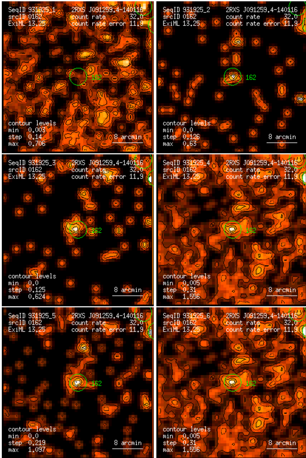
Figure 162: RASS 931925: detection 0162: band rate images, Gaussian filter: (1) PSPC channels 11 – 41, (2) 52 – 90, (3) 91 – 201, (4) 11 – 235, (5) 52 – 201, (6) 11 – 201. Broad band rates in counts/ks. Band rate contour levels in counts/ks/arcmin 2 .
