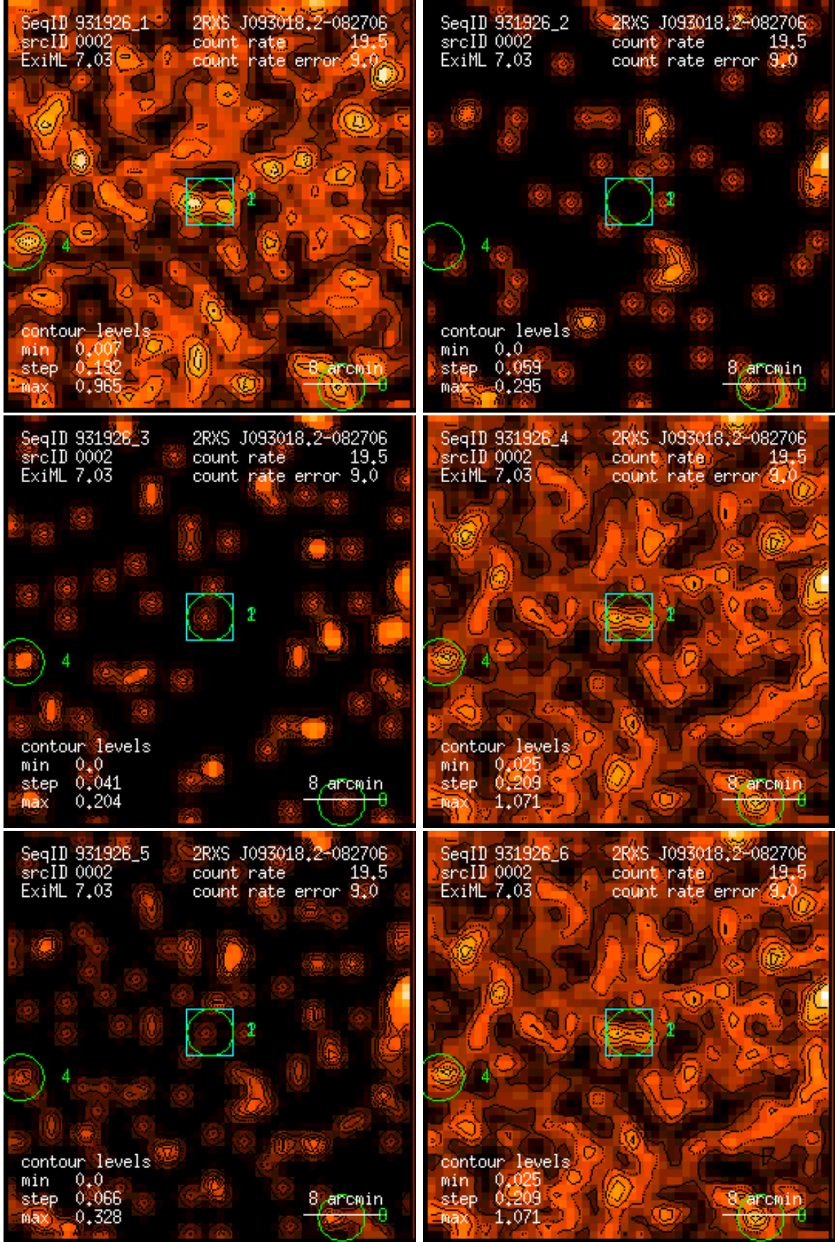
Figure 2: RASS 931926: detection 0002: band rate images, Gaussian filter: (1) PSPC channels 11 – 41, (2) 52 – 90, (3) 91 – 201, (4) 11 – 235, (5) 52 – 201, (6) 11 – 201. Broad band rates in counts/ks. Band rate contour levels in counts/ks/arcmin 2 .
