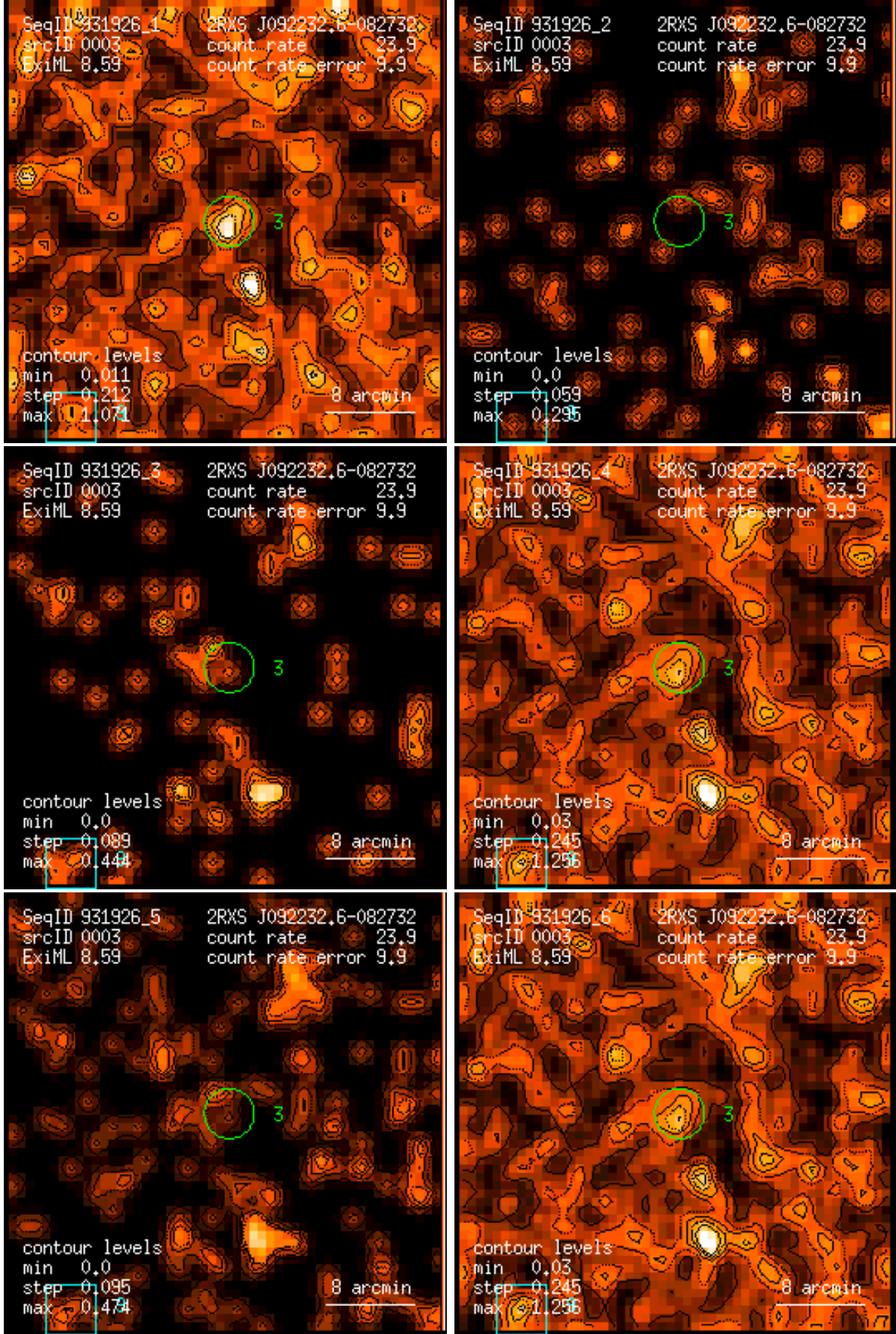
Figure 3: RASS 931926: detection 0003: band rate images, Gaussian filter: (1) PSPC channels 11 – 41, (2) 52 – 90, (3) 91 – 201, (4) 11 – 235, (5) 52 – 201, (6) 11 – 201. Broad band rates in counts/ks. Band rate contour levels in counts/ks/arcmin 2 .
