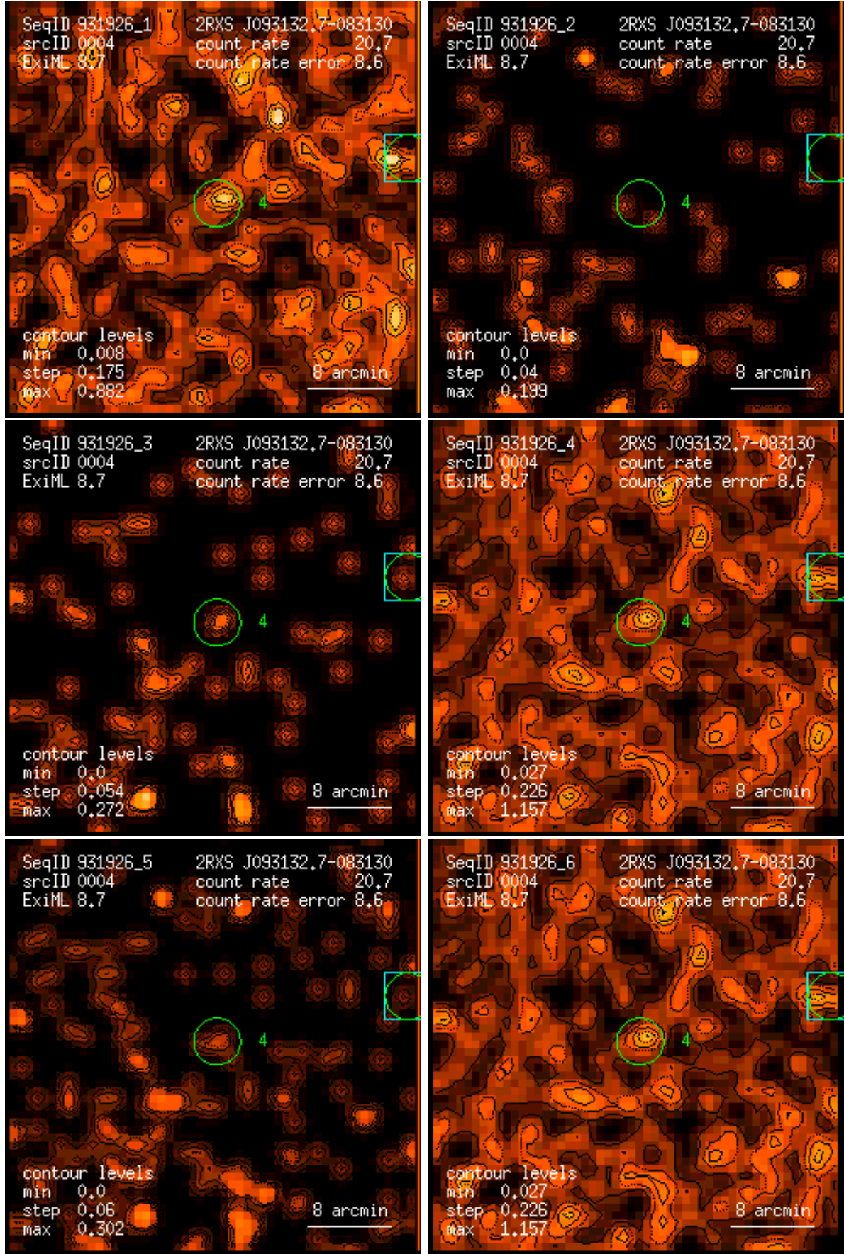
Figure 4: RASS 931926: detection 0004: band rate images, Gaussian filter: (1) PSPC channels 11 – 41, (2) 52 – 90, (3) 91 – 201, (4) 11 – 235, (5) 52 – 201, (6) 11 – 201. Broad band rates in counts/ks. Band rate contour levels in counts/ks/arcmin 2 .
