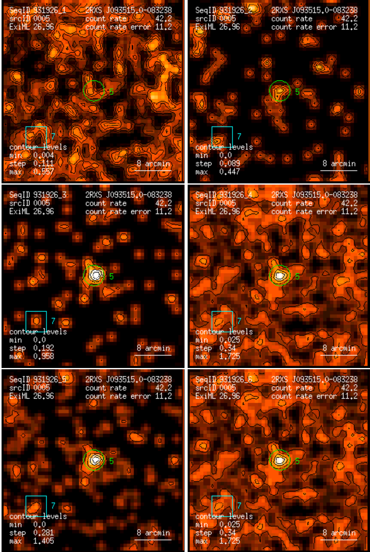
Figure 5: RASS 931926: detection 0005: band rate images, Gaussian filter: (1) PSPC channels 11 – 41, (2) 52 – 90, (3) 91 – 201, (4) 11 – 235, (5) 52 – 201, (6) 11 – 201. Broad band rates in counts/ks. Band rate contour levels in counts/ks/arcmin 2 .
