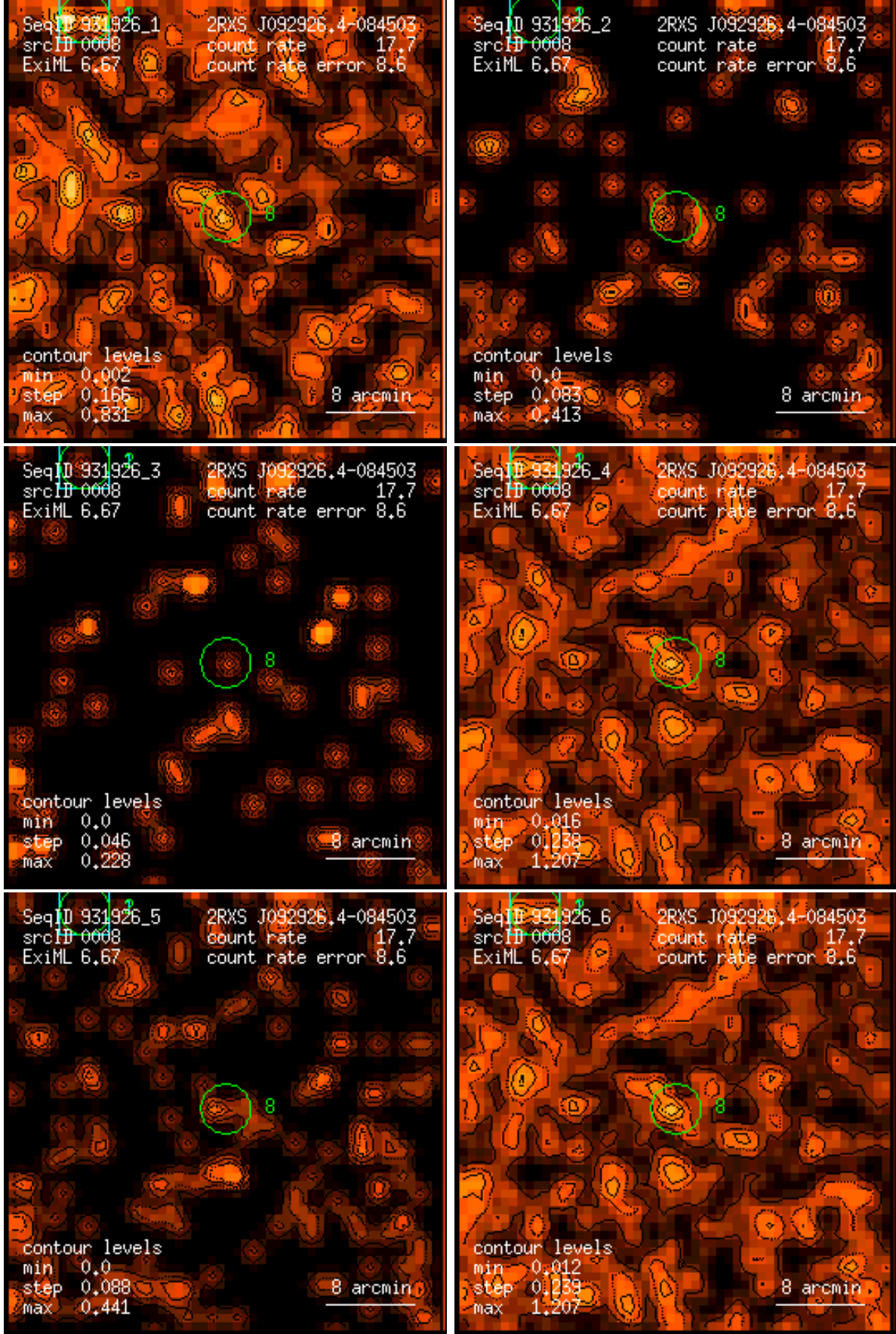
Figure 8: RASS 931926: detection 0008: band rate images, Gaussian filter: (1) PSPC channels 11 – 41, (2) 52 – 90, (3) 91 – 201, (4) 11 – 235, (5) 52 – 201, (6) 11 – 201. Broad band rates in counts/ks. Band rate contour levels in counts/ks/arcmin 2 .
