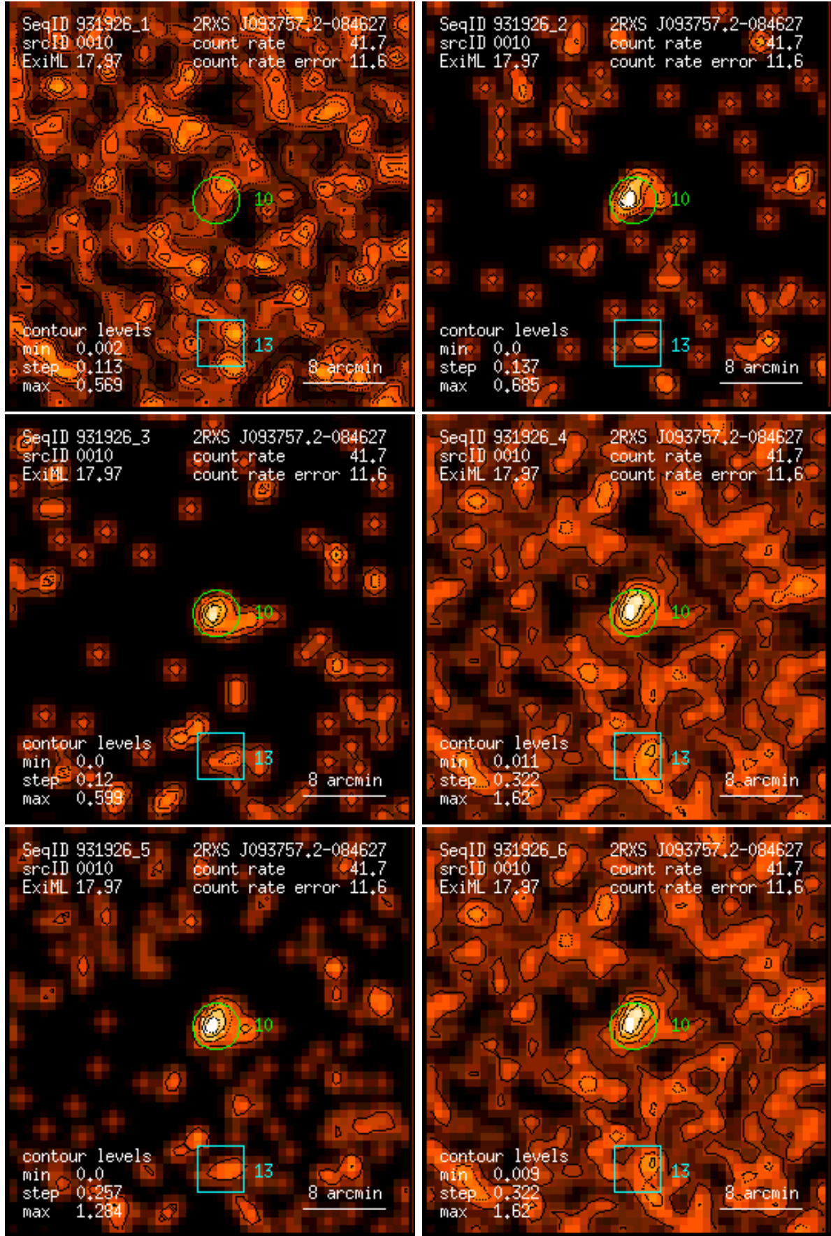
Figure 10: RASS 931926: detection 0010: band rate images, Gaussian filter: (1) PSPC channels 11 – 41, (2) 52 – 90, (3) 91 – 201, (4) 11 – 235, (5) 52 – 201, (6) 11 – 201. Broad band rates in counts/ks. Band rate contour levels in counts/ks/arcmin 2 .
