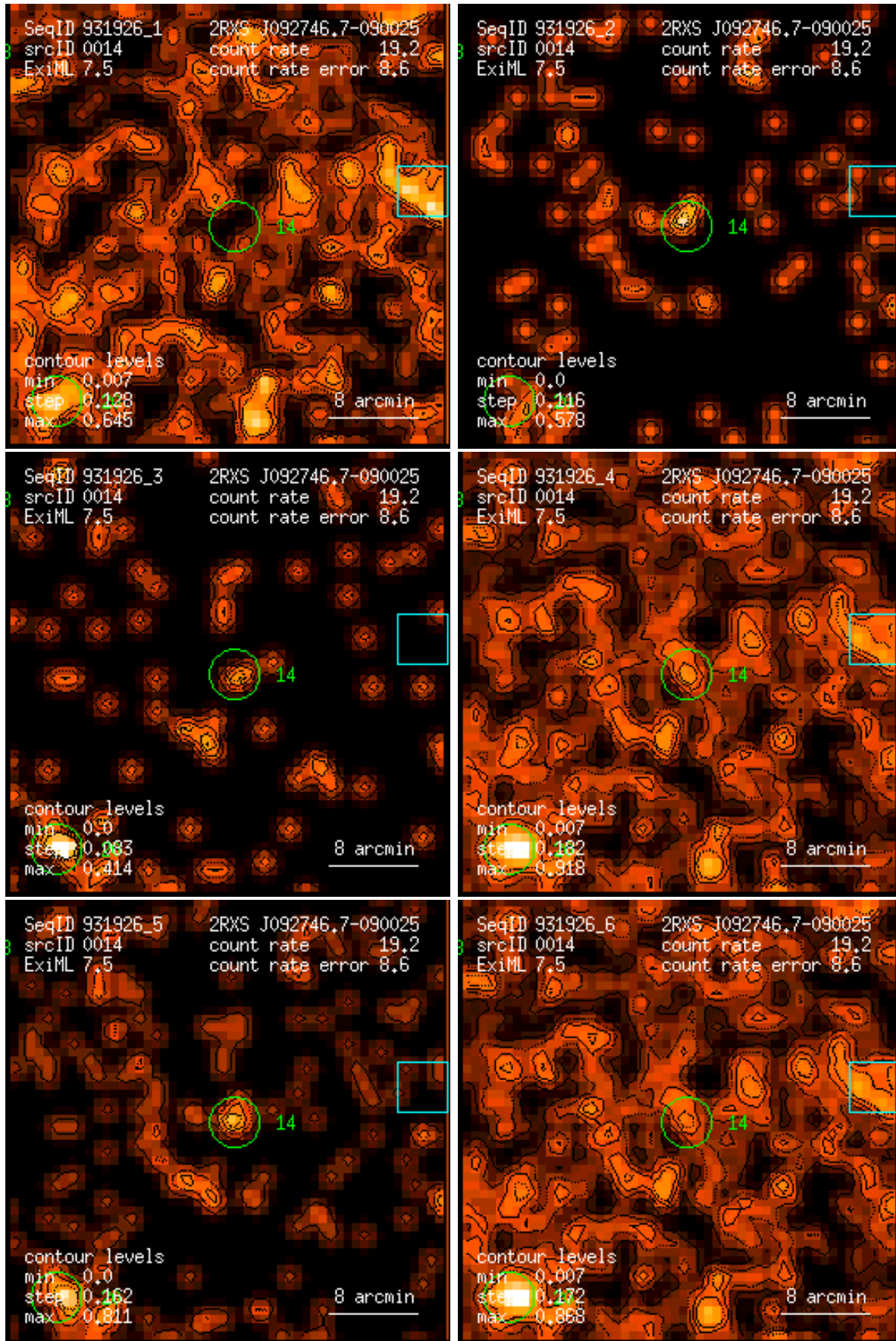
Figure 14: RASS 931926: detection 0014: band rate images, Gaussian filter: (1) PSPC channels 11 – 41, (2) 52 – 90, (3) 91 – 201, (4) 11 – 235, (5) 52 – 201, (6) 11 – 201. Broad band rates in counts/ks. Band rate contour levels in counts/ks/arcmin 2 .
