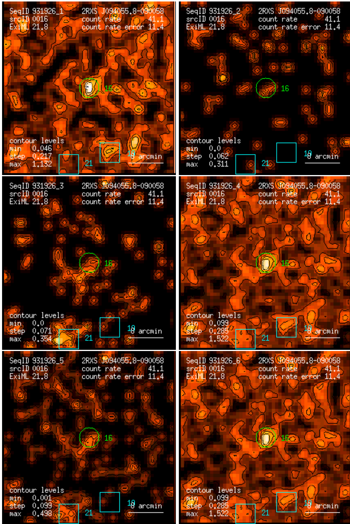
Figure 16: RASS 931926: detection 0016: band rate images, Gaussian filter: (1) PSPC channels 11 – 41, (2) 52 – 90, (3) 91 – 201, (4) 11 – 235, (5) 52 – 201, (6) 11 – 201. Broad band rates in counts/ks. Band rate contour levels in counts/ks/arcmin 2 .
