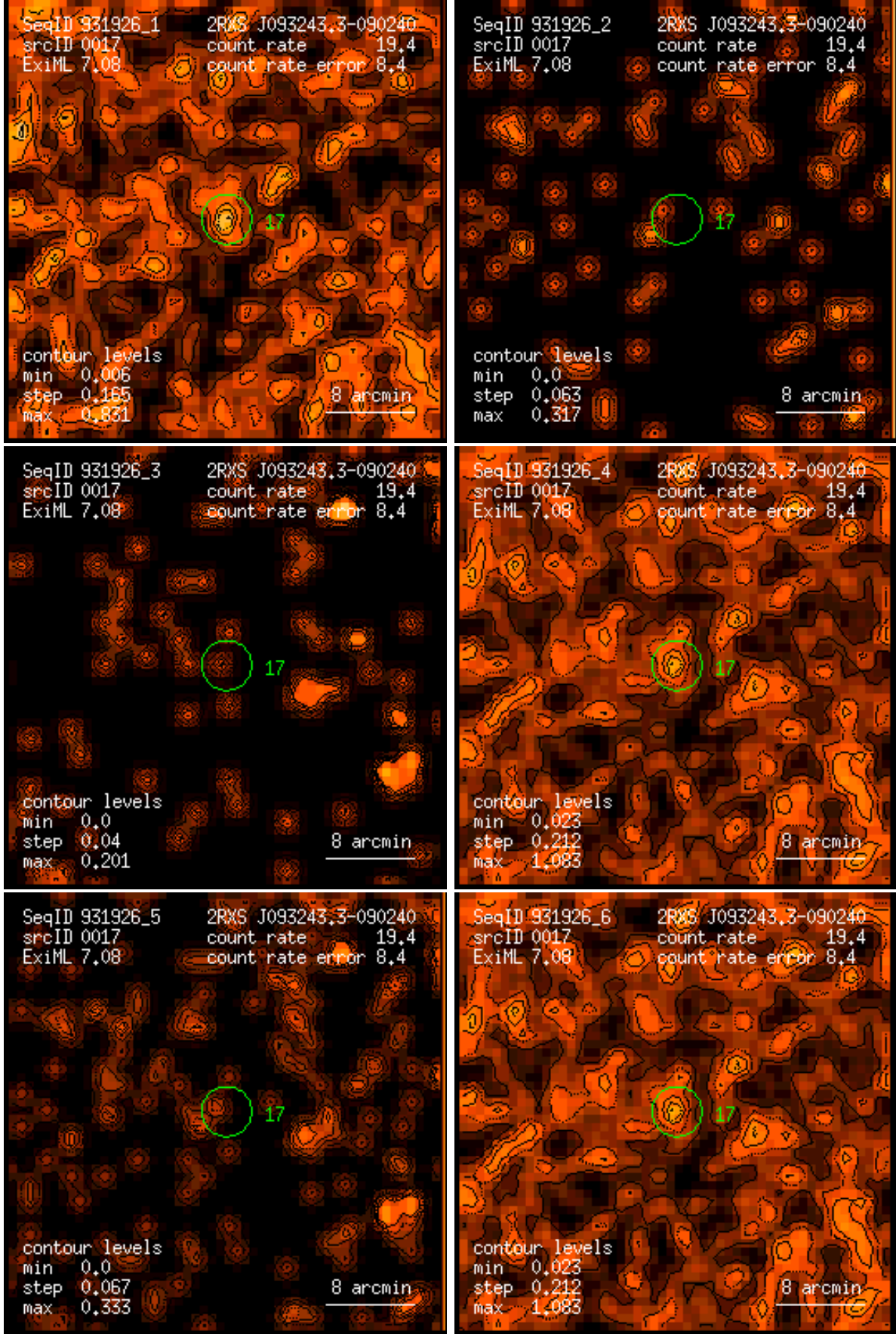
Figure 17: RASS 931926: detection 0017: band rate images, Gaussian filter: (1) PSPC channels 11 – 41, (2) 52 – 90, (3) 91 – 201, (4) 11 – 235, (5) 52 – 201, (6) 11 – 201. Broad band rates in counts/ks. Band rate contour levels in counts/ks/arcmin 2 .
