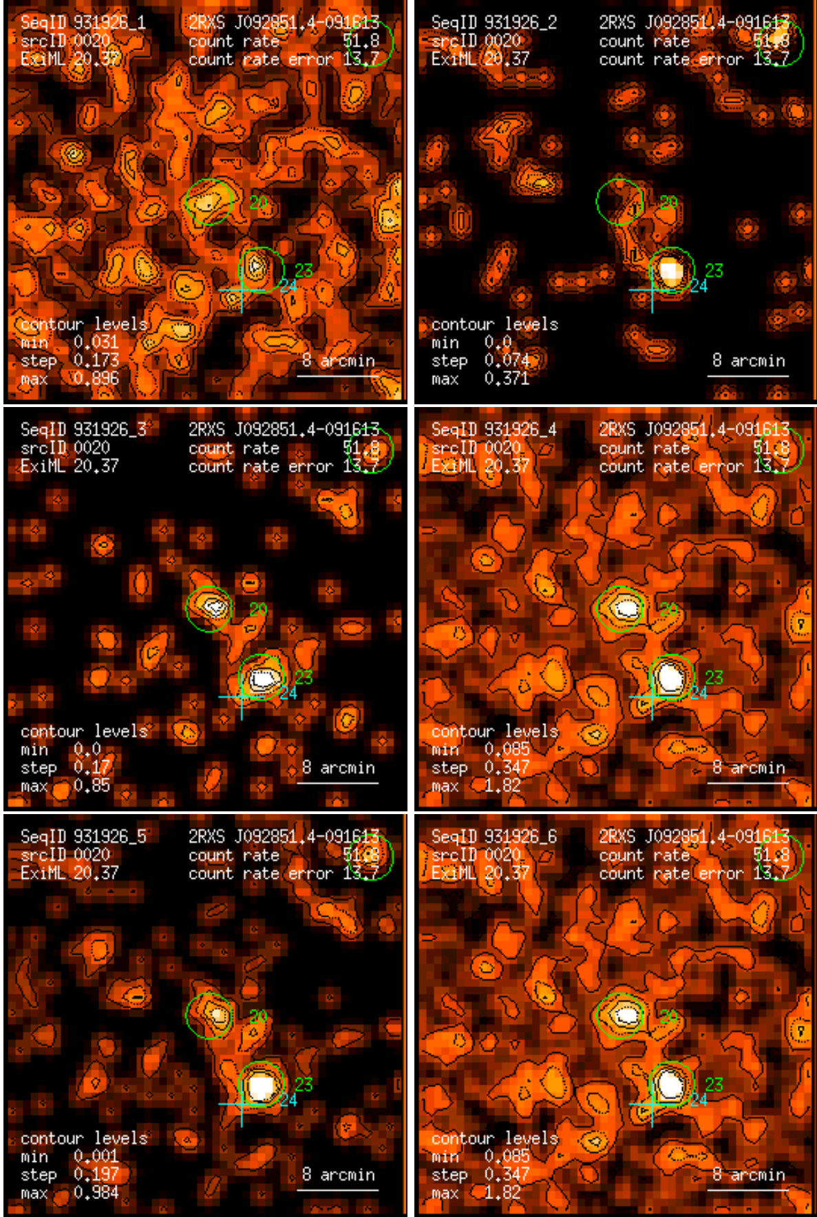
Figure 20: RASS 931926: detection 0020: band rate images, Gaussian filter: (1) PSPC channels 11 – 41, (2) 52 – 90, (3) 91 – 201, (4) 11 – 235, (5) 52 – 201, (6) 11 – 201. Broad band rates in counts/ks. Band rate contour levels in counts/ks/arcmin 2 .
