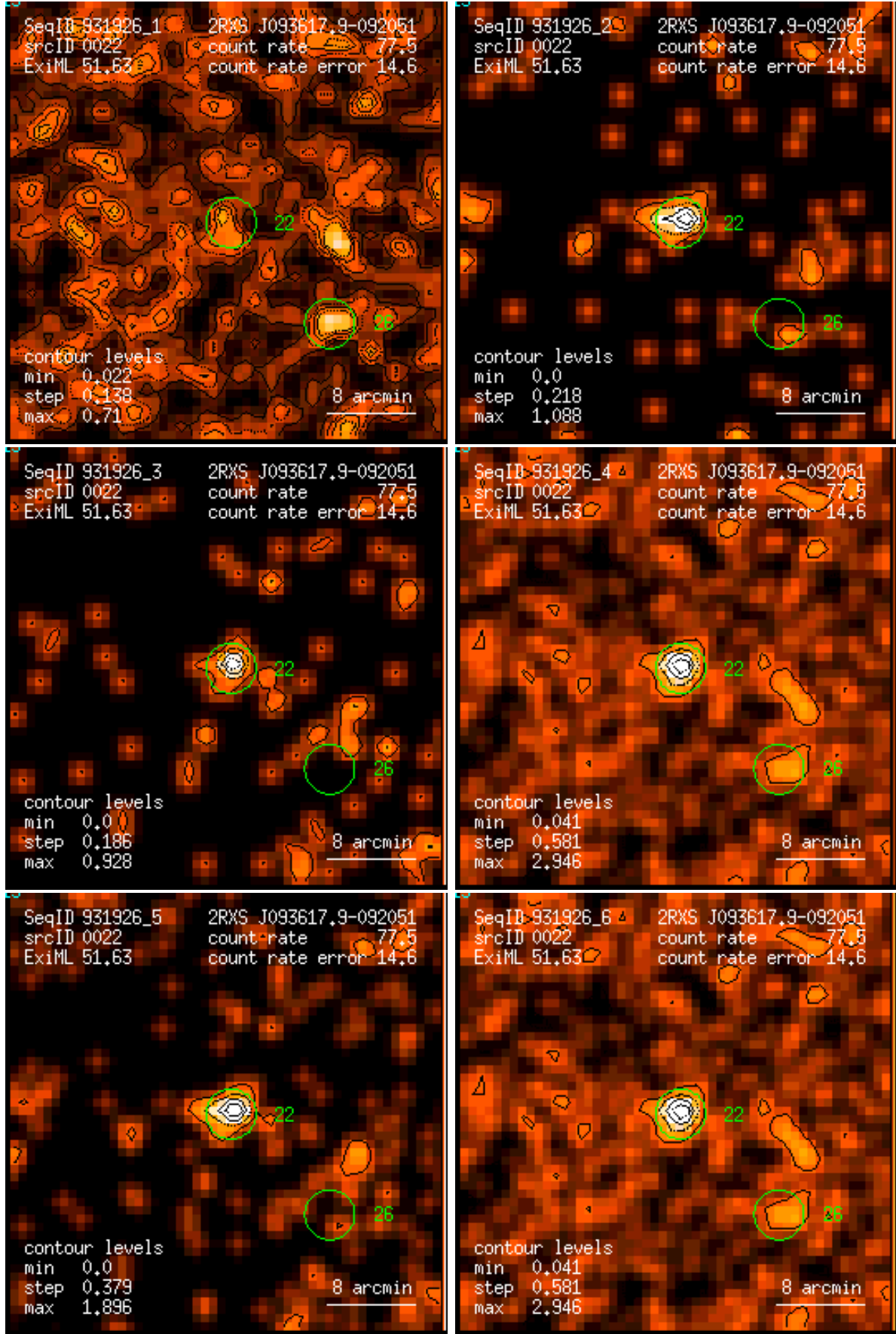
Figure 22: RASS 931926: detection 0022: band rate images, Gaussian filter: (1) PSPC channels 11 – 41, (2) 52 – 90, (3) 91 – 201, (4) 11 – 235, (5) 52 – 201, (6) 11 – 201. Broad band rates in counts/ks. Band rate contour levels in counts/ks/arcmin 2 .
