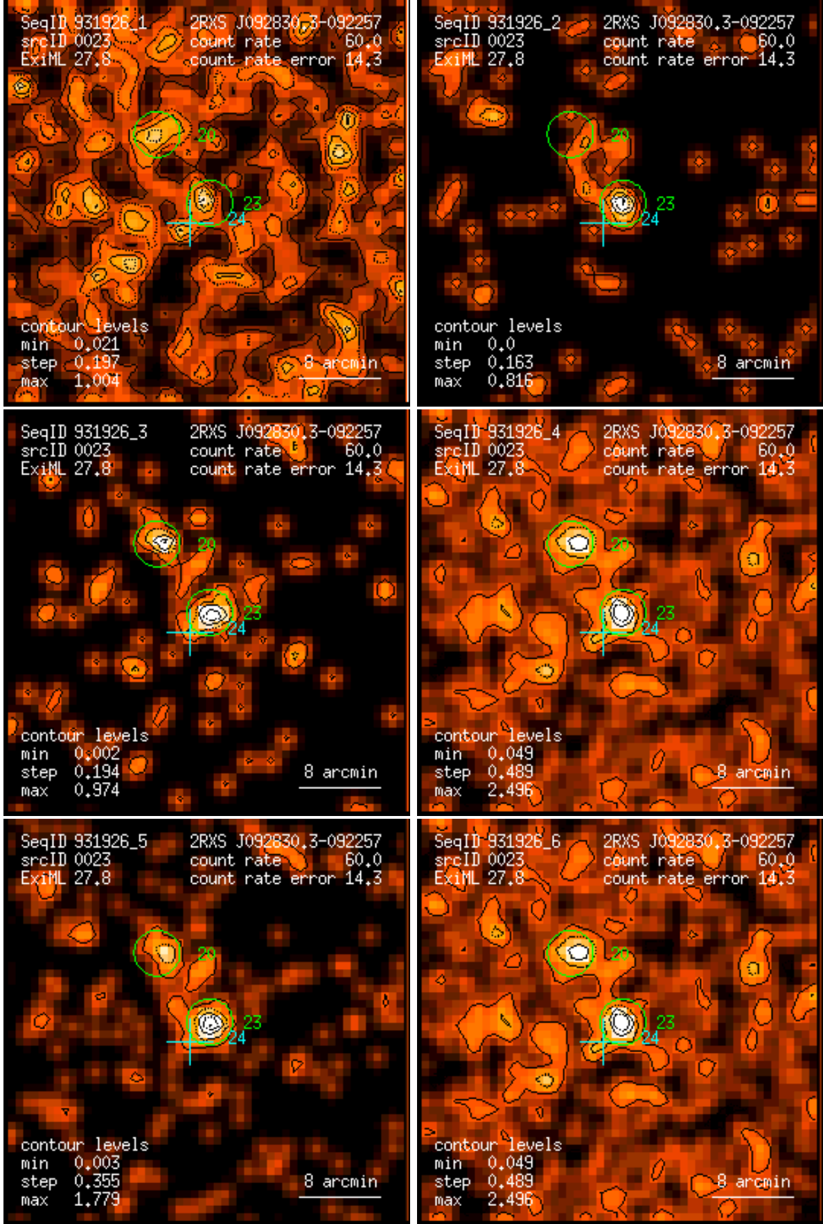
Figure 23: RASS 931926: detection 0023: band rate images, Gaussian filter: (1) PSPC channels 11 – 41, (2) 52 – 90, (3) 91 – 201, (4) 11 – 235, (5) 52 – 201, (6) 11 – 201. Broad band rates in counts/ks. Band rate contour levels in counts/ks/arcmin 2 .
