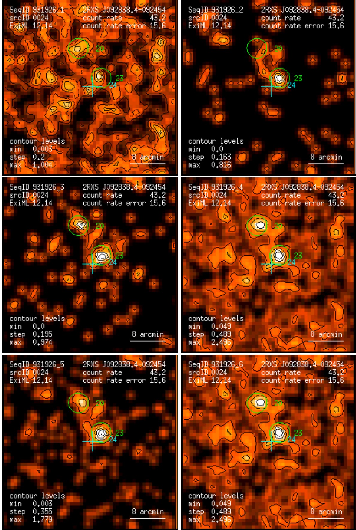
Figure 24: RASS 931926: detection 0024: band rate images, Gaussian filter: (1) PSPC channels 11 – 41, (2) 52 – 90, (3) 91 – 201, (4) 11 – 235, (5) 52 – 201, (6) 11 – 201. Broad band rates in counts/ks. Band rate contour levels in counts/ks/arcmin 2 .
