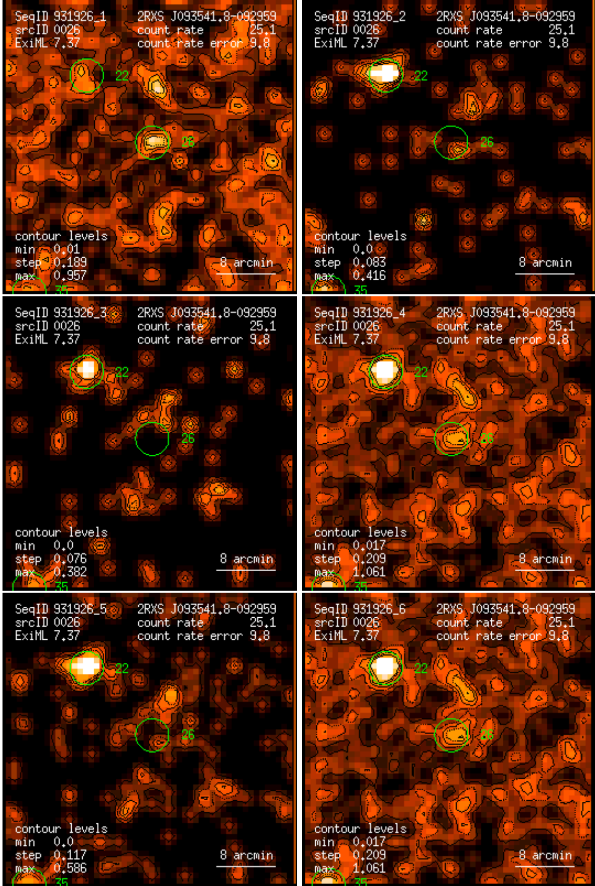
Figure 26: RASS 931926: detection 0026: band rate images, Gaussian filter: (1) PSPC channels 11 – 41, (2) 52 – 90, (3) 91 – 201, (4) 11 – 235, (5) 52 – 201, (6) 11 – 201. Broad band rates in counts/ks. Band rate contour levels in counts/ks/arcmin 2 .
