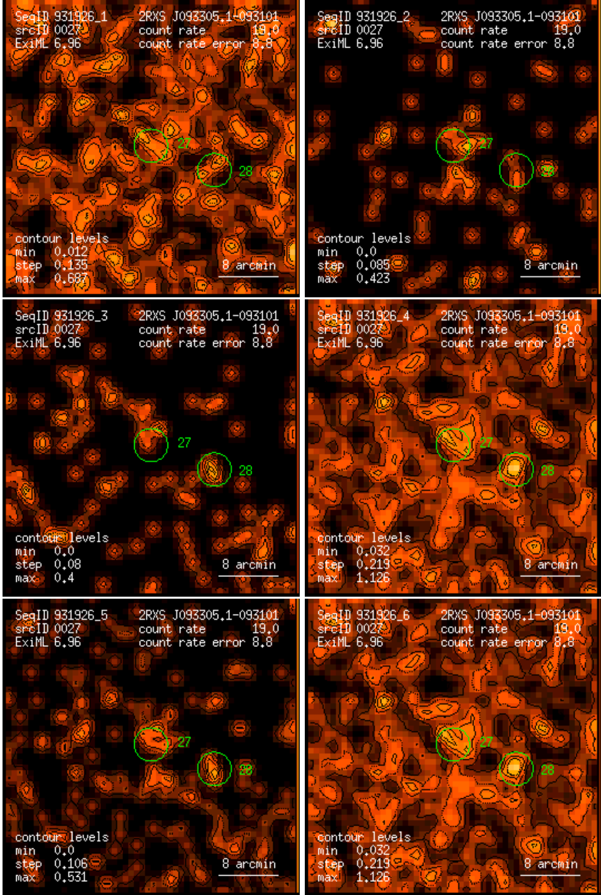
Figure 27: RASS 931926: detection 0027: band rate images, Gaussian filter: (1) PSPC channels 11 – 41, (2) 52 – 90, (3) 91 – 201, (4) 11 – 235, (5) 52 – 201, (6) 11 – 201. Broad band rates in counts/ks. Band rate contour levels in counts/ks/arcmin 2 .
