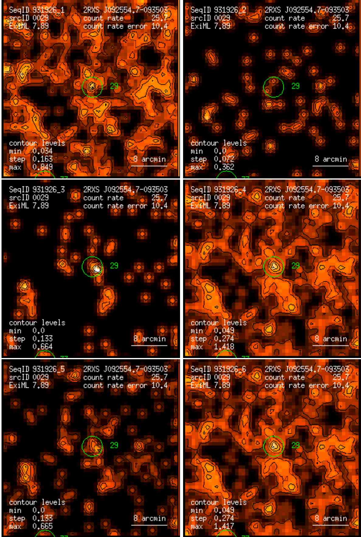
Figure 29: RASS 931926: detection 0029: band rate images, Gaussian filter: (1) PSPC channels 11 – 41, (2) 52 – 90, (3) 91 – 201, (4) 11 – 235, (5) 52 – 201, (6) 11 – 201. Broad band rates in counts/ks. Band rate contour levels in counts/ks/arcmin 2 .
