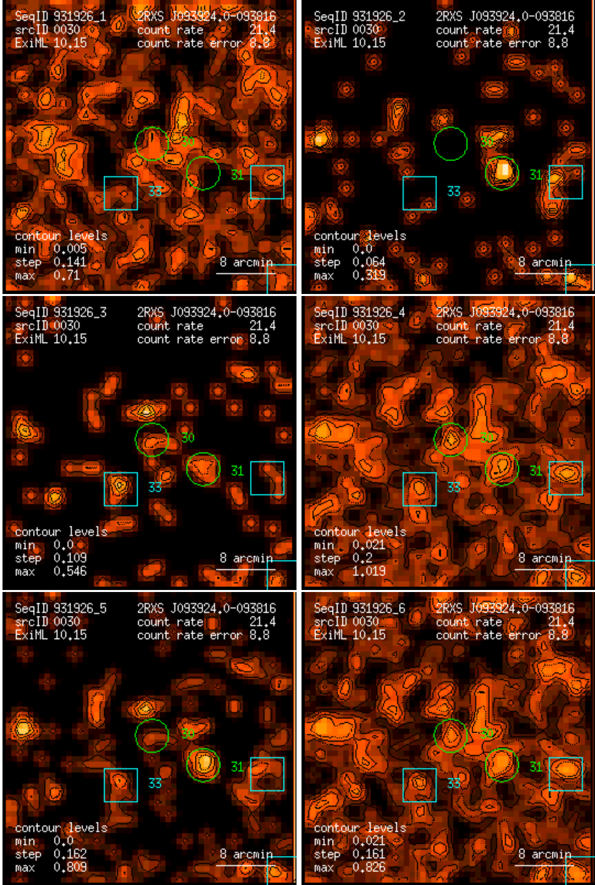
Figure 30: RASS 931926: detection 0030: band rate images, Gaussian filter: (1) PSPC channels 11 – 41, (2) 52 – 90, (3) 91 – 201, (4) 11 – 235, (5) 52 – 201, (6) 11 – 201. Broad band rates in counts/ks. Band rate contour levels in counts/ks/arcmin 2 .
