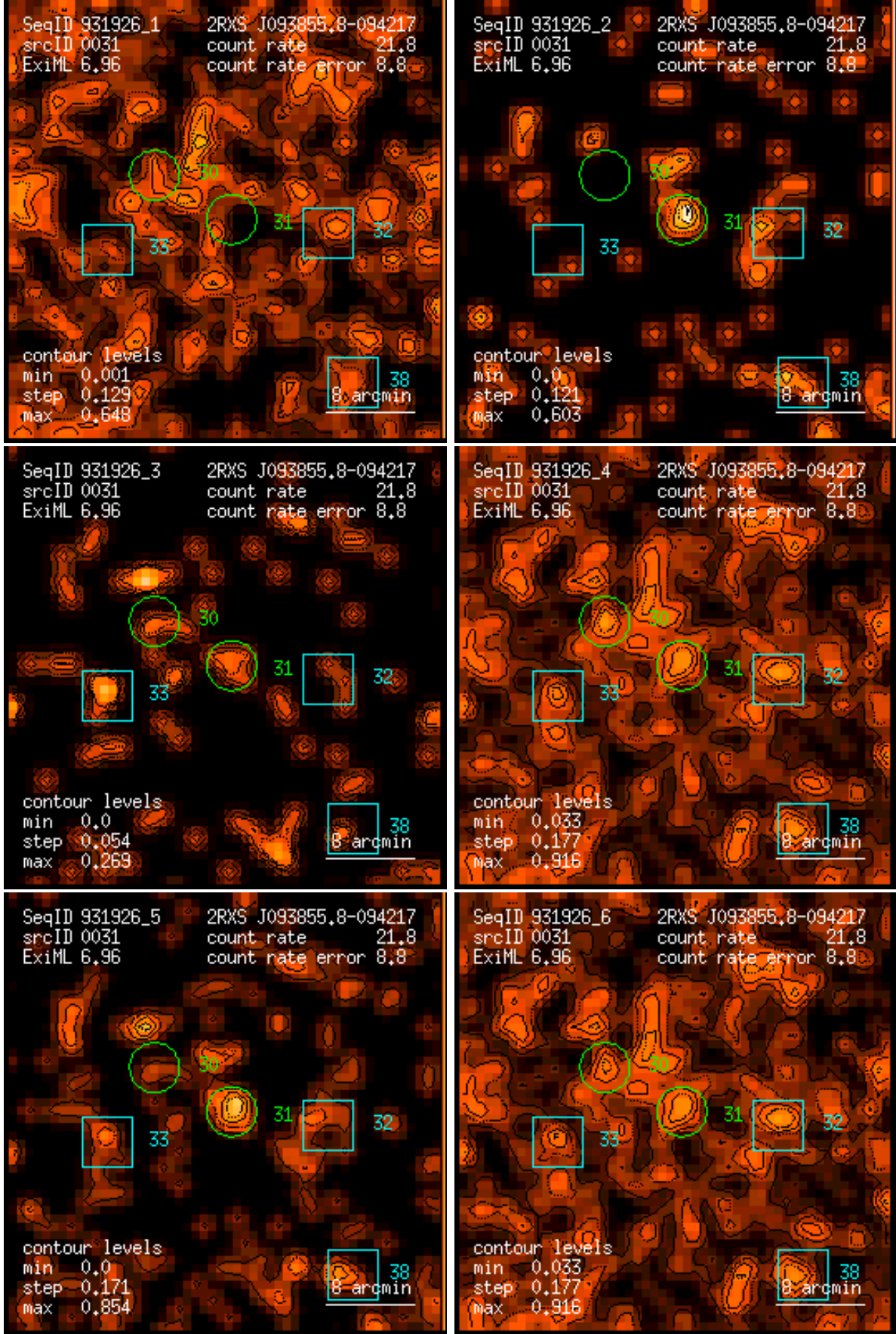
Figure 31: RASS 931926: detection 0031: band rate images, Gaussian filter: (1) PSPC channels 11 – 41, (2) 52 – 90, (3) 91 – 201, (4) 11 – 235, (5) 52 – 201, (6) 11 – 201. Broad band rates in counts/ks. Band rate contour levels in counts/ks/arcmin 2 .
