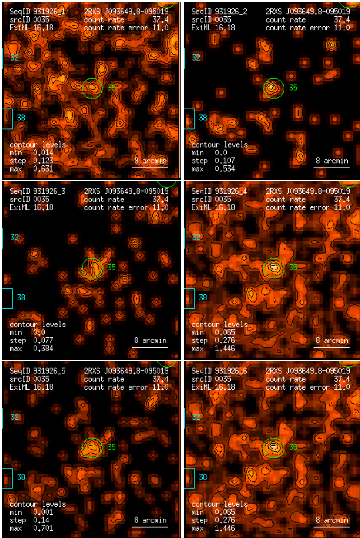
Figure 35: RASS 931926: detection 0035: band rate images, Gaussian filter: (1) PSPC channels 11 – 41, (2) 52 – 90, (3) 91 – 201, (4) 11 – 235, (5) 52 – 201, (6) 11 – 201. Broad band rates in counts/ks. Band rate contour levels in counts/ks/arcmin 2 .
