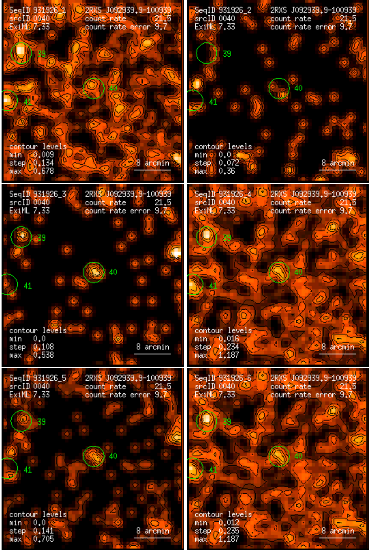
Figure 40: RASS 931926: detection 0040: band rate images, Gaussian filter: (1) PSPC channels 11 – 41, (2) 52 – 90, (3) 91 – 201, (4) 11 – 235, (5) 52 – 201, (6) 11 – 201. Broad band rates in counts/ks. Band rate contour levels in counts/ks/arcmin 2 .
