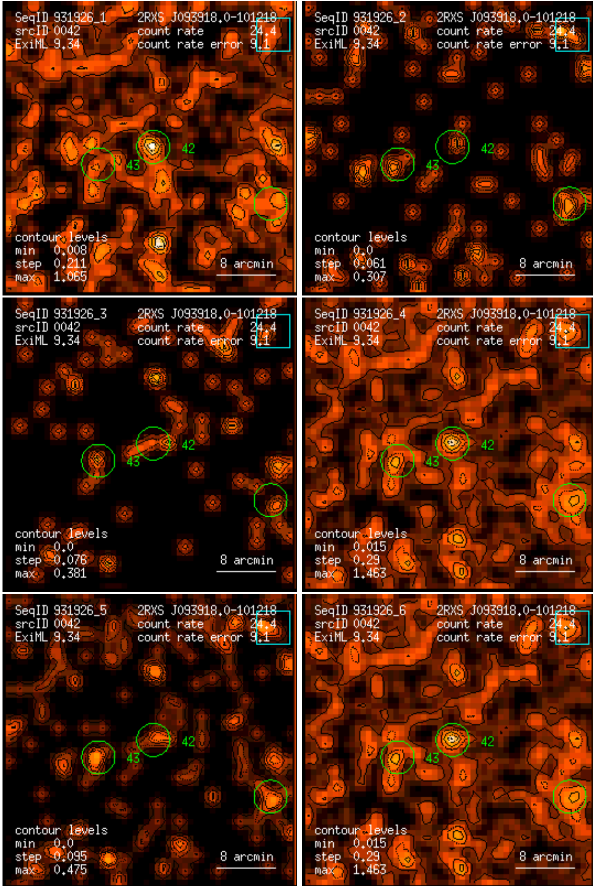
Figure 42: RASS 931926: detection 0042: band rate images, Gaussian filter: (1) PSPC channels 11 – 41, (2) 52 – 90, (3) 91 – 201, (4) 11 – 235, (5) 52 – 201, (6) 11 – 201. Broad band rates in counts/ks. Band rate contour levels in counts/ks/arcmin 2 .
