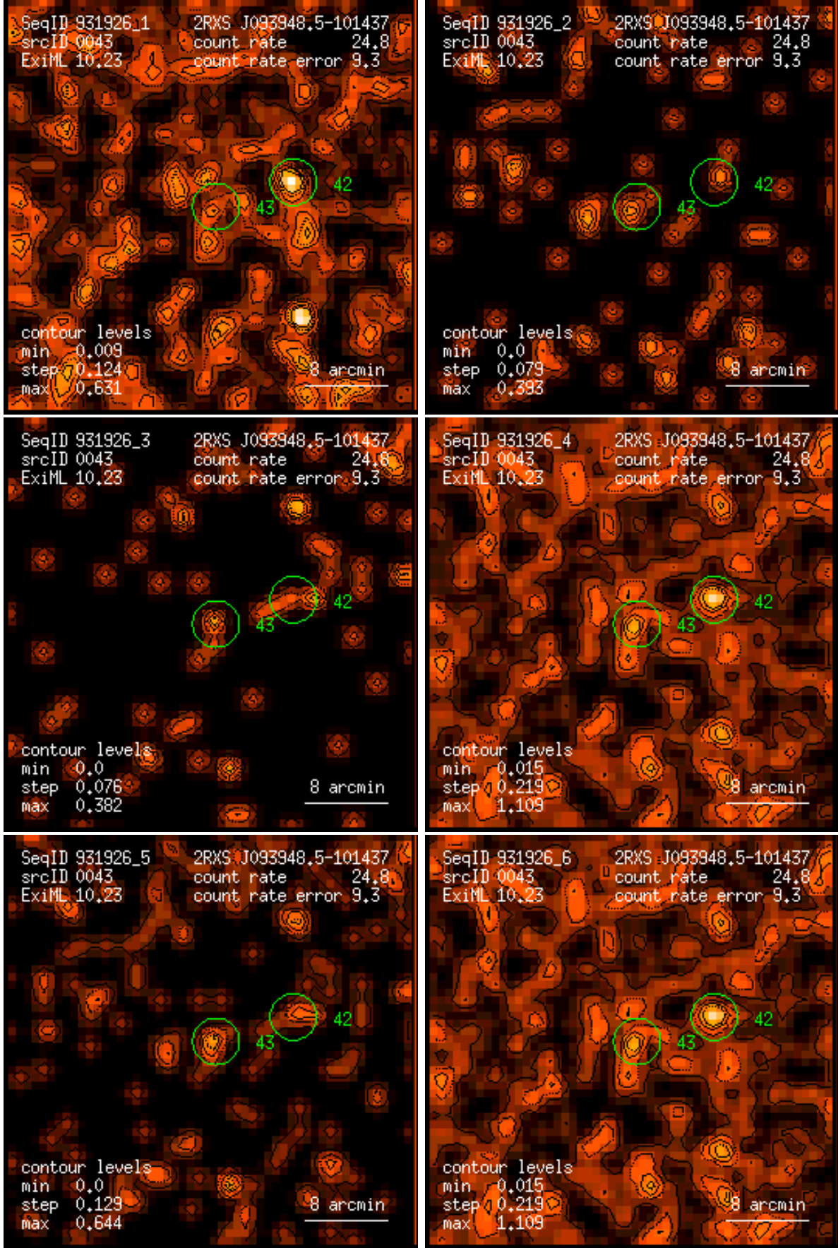
Figure 43: RASS 931926: detection 0043: band rate images, Gaussian filter: (1) PSPC channels 11 – 41, (2) 52 – 90, (3) 91 – 201, (4) 11 – 235, (5) 52 – 201, (6) 11 – 201. Broad band rates in counts/ks. Band rate contour levels in counts/ks/arcmin 2 .
