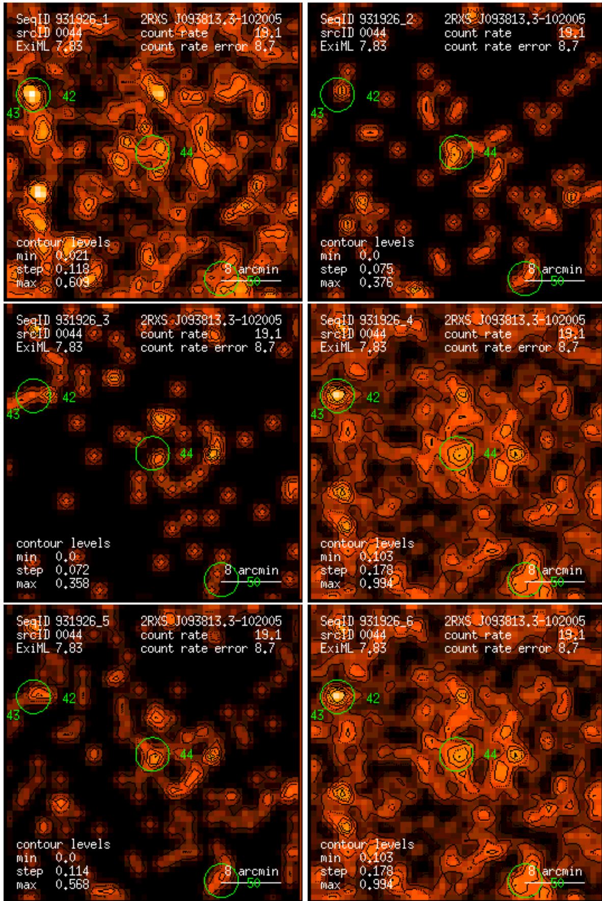
Figure 44: RASS 931926: detection 0044: band rate images, Gaussian filter: (1) PSPC channels 11 – 41, (2) 52 – 90, (3) 91 – 201, (4) 11 – 235, (5) 52 – 201, (6) 11 – 201. Broad band rates in counts/ks. Band rate contour levels in counts/ks/arcmin 2 .
