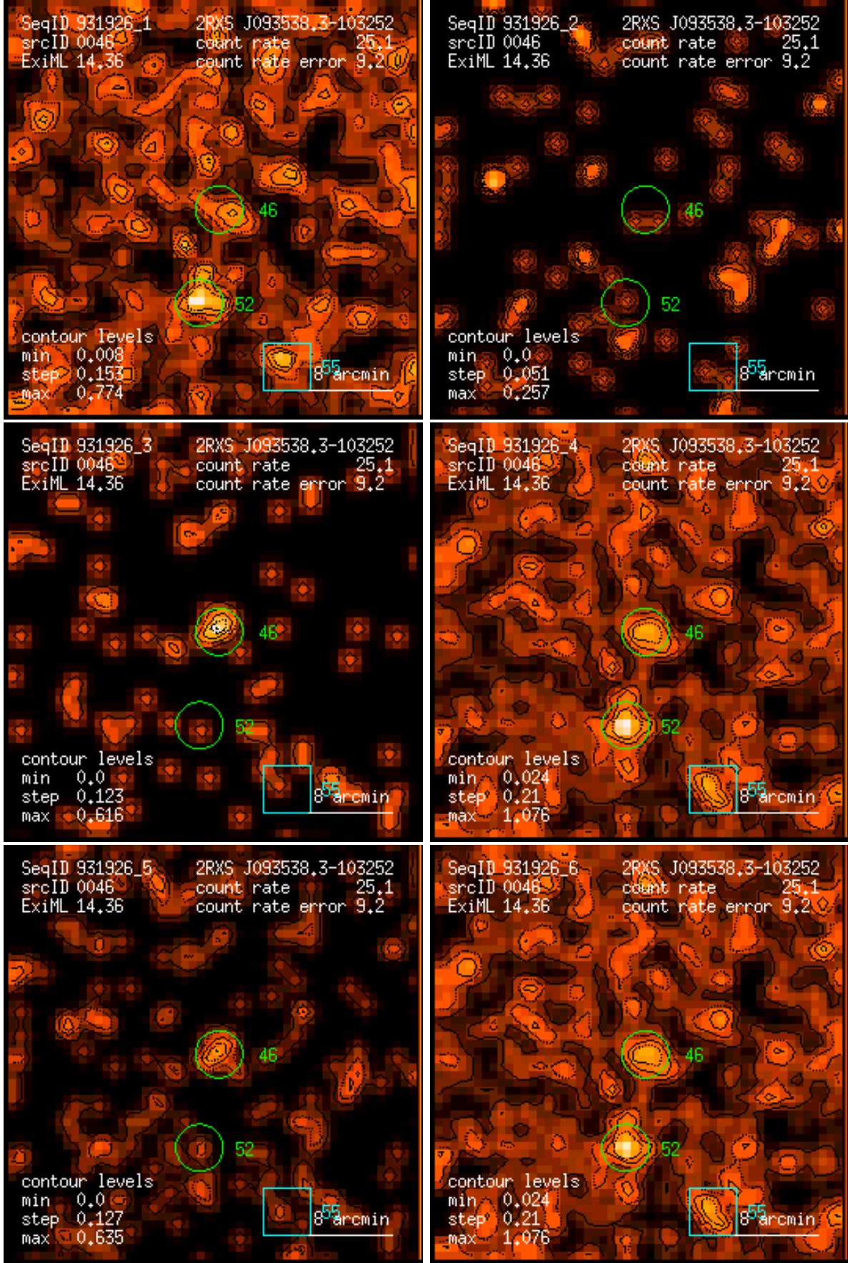
Figure 46: RASS 931926: detection 0046: band rate images, Gaussian filter: (1) PSPC channels 11 – 41, (2) 52 – 90, (3) 91 – 201, (4) 11 – 235, (5) 52 – 201, (6) 11 – 201. Broad band rates in counts/ks. Band rate contour levels in counts/ks/arcmin 2 .
