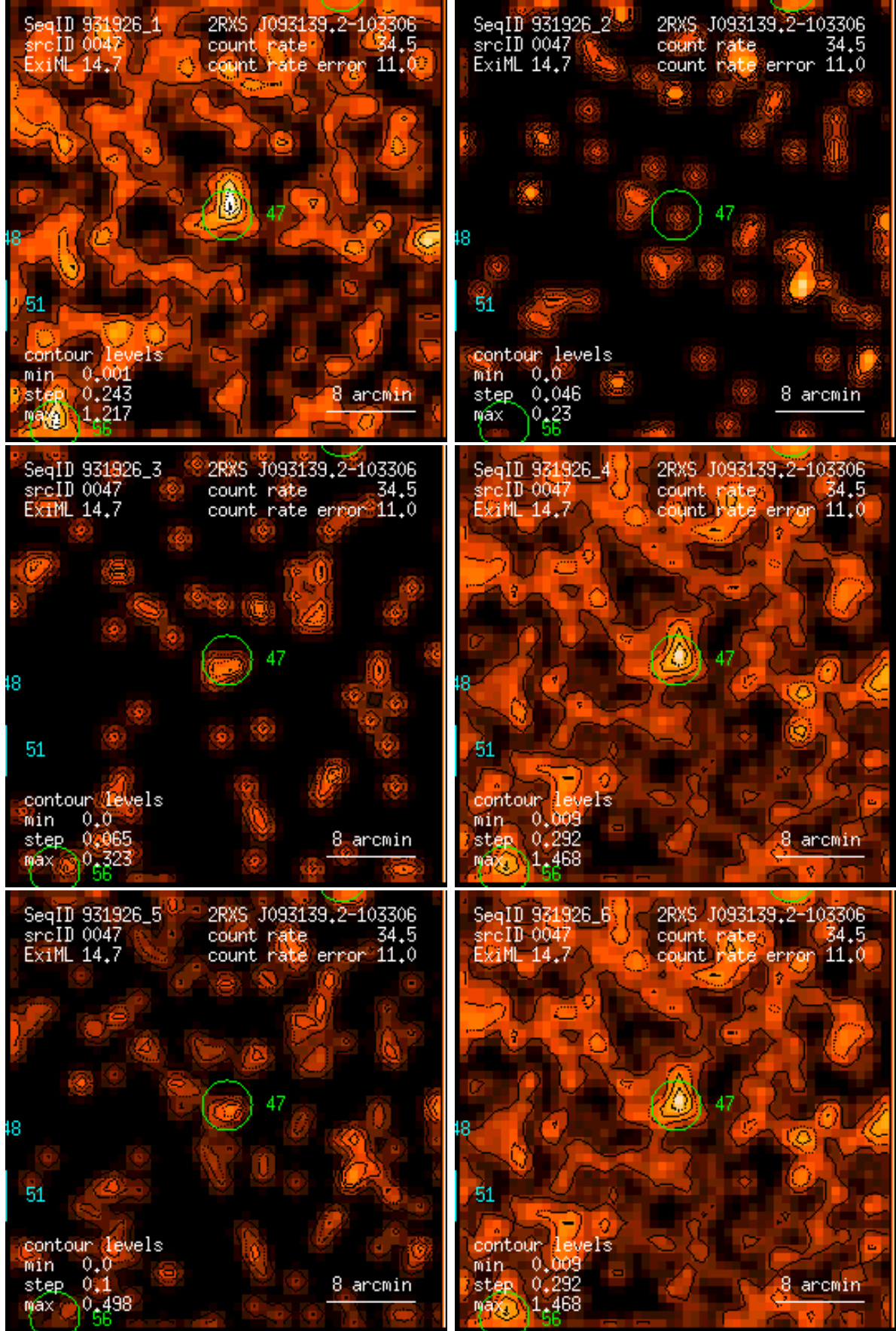
Figure 47: RASS 931926: detection 0047: band rate images, Gaussian filter: (1) PSPC channels 11 – 41, (2) 52 – 90, (3) 91 – 201, (4) 11 – 235, (5) 52 – 201, (6) 11 – 201. Broad band rates in counts/ks. Band rate contour levels in counts/ks/arcmin 2 .
