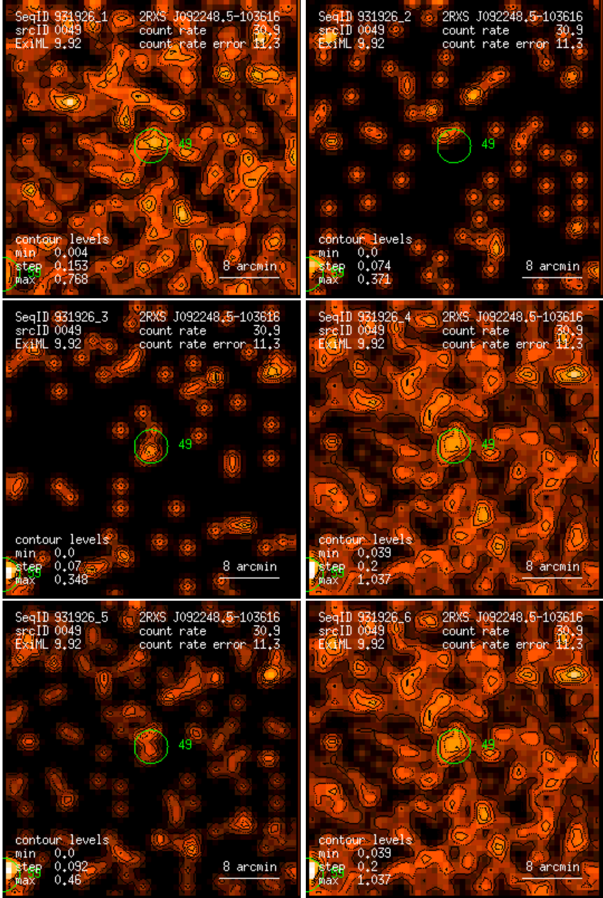
Figure 49: RASS 931926: detection 0049: band rate images, Gaussian filter: (1) PSPC channels 11 – 41, (2) 52 – 90, (3) 91 – 201, (4) 11 – 235, (5) 52 – 201, (6) 11 – 201. Broad band rates in counts/ks. Band rate contour levels in counts/ks/arcmin 2 .
