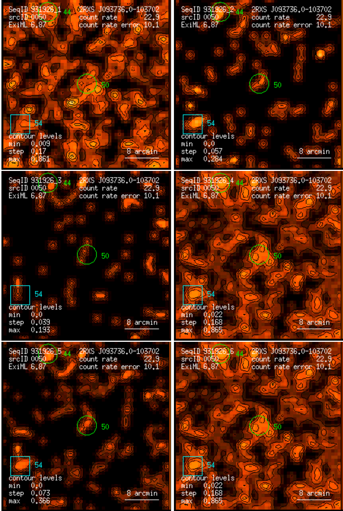
Figure 50: RASS 931926: detection 0050: band rate images, Gaussian filter: (1) PSPC channels 11 – 41, (2) 52 – 90, (3) 91 – 201, (4) 11 – 235, (5) 52 – 201, (6) 11 – 201. Broad band rates in counts/ks. Band rate contour levels in counts/ks/arcmin 2 .
