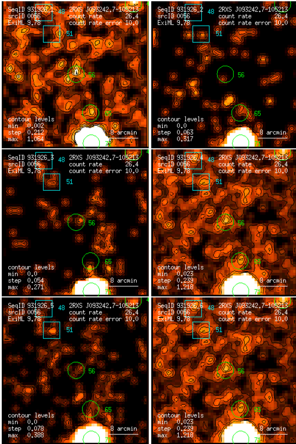
Figure 56: RASS 931926: detection 0056: band rate images, Gaussian filter: (1) PSPC channels 11 – 41, (2) 52 – 90, (3) 91 – 201, (4) 11 – 235, (5) 52 – 201, (6) 11 – 201. Broad band rates in counts/ks. Band rate contour levels in counts/ks/arcmin 2 .
