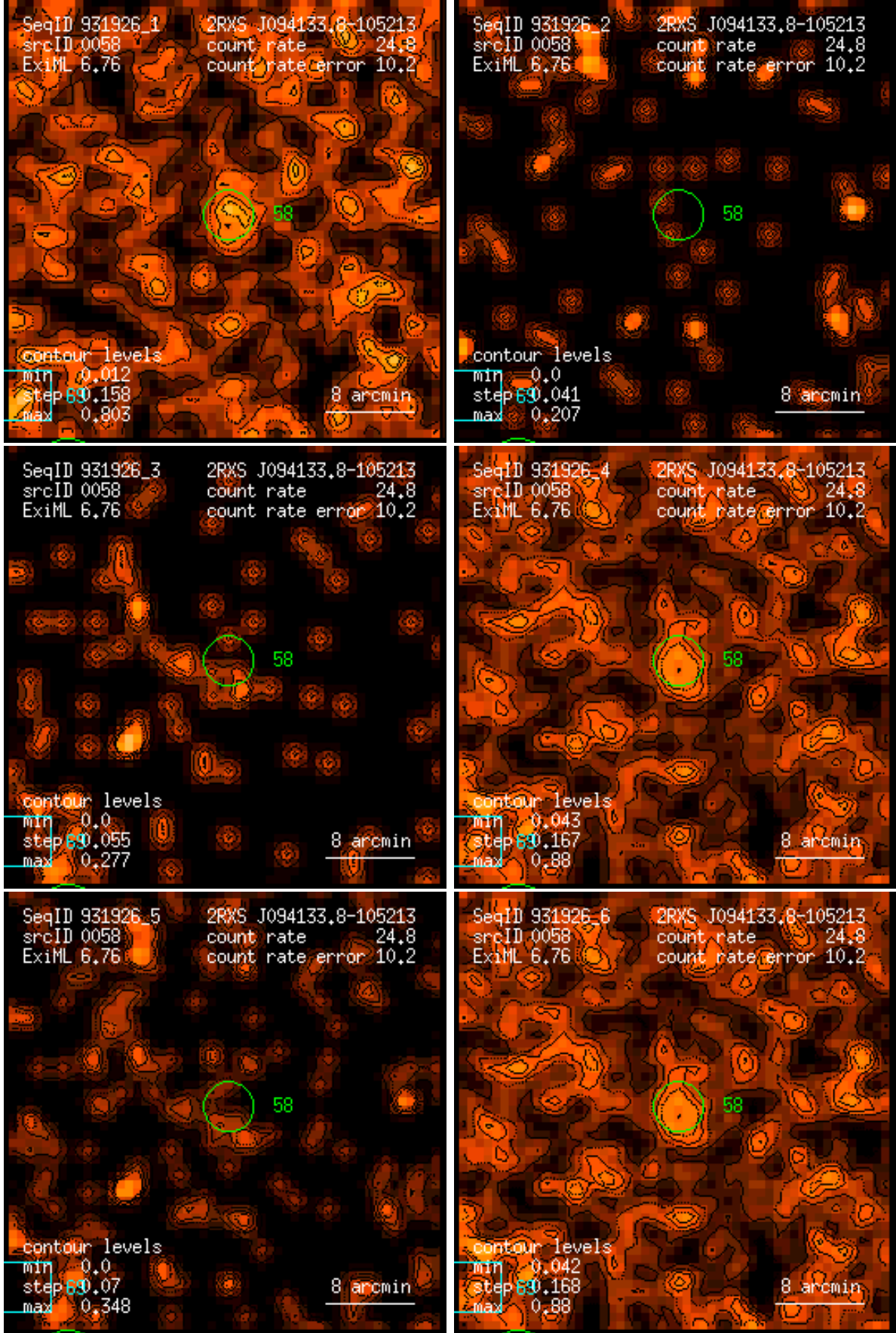
Figure 58: RASS 931926: detection 0058: band rate images, Gaussian filter: (1) PSPC channels 11 – 41, (2) 52 – 90, (3) 91 – 201, (4) 11 – 235, (5) 52 – 201, (6) 11 – 201. Broad band rates in counts/ks. Band rate contour levels in counts/ks/arcmin 2 .
