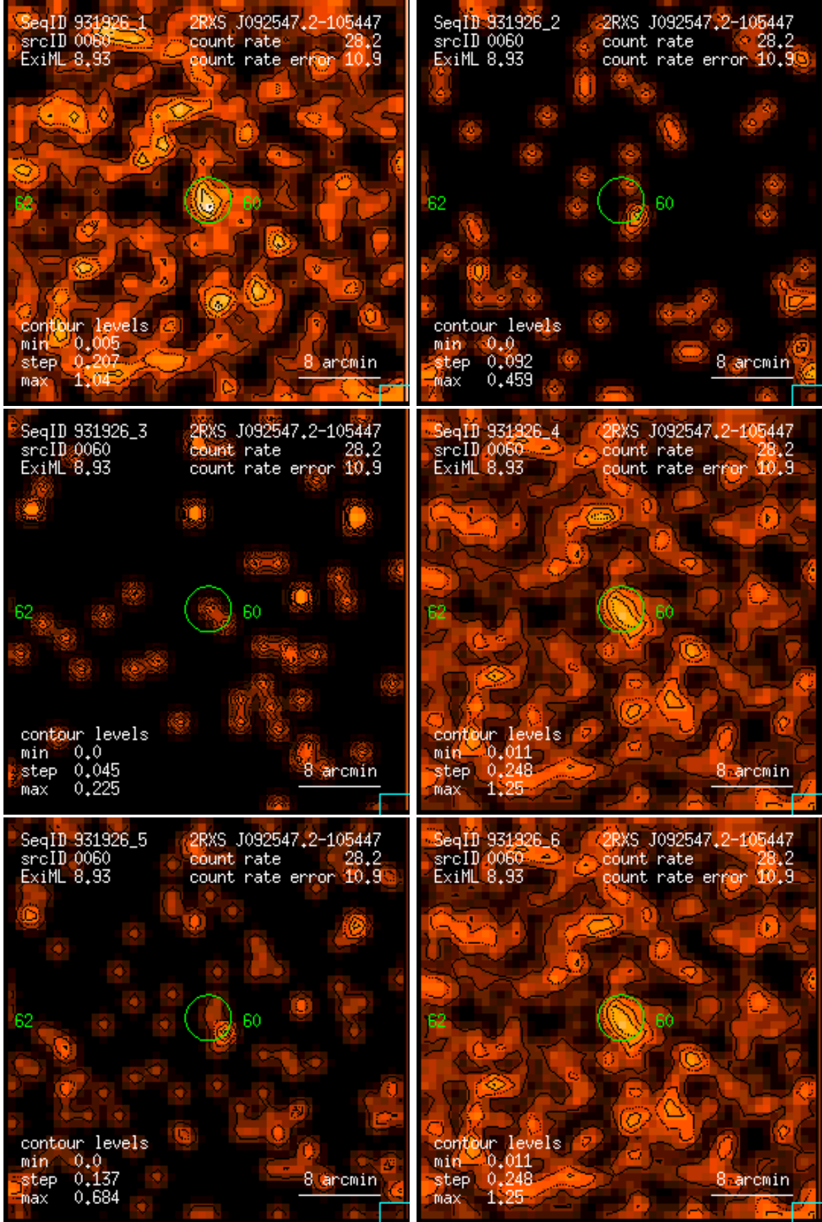
Figure 60: RASS 931926: detection 0060: band rate images, Gaussian filter: (1) PSPC channels 11 – 41, (2) 52 – 90, (3) 91 – 201, (4) 11 – 235, (5) 52 – 201, (6) 11 – 201. Broad band rates in counts/ks. Band rate contour levels in counts/ks/arcmin 2 .
