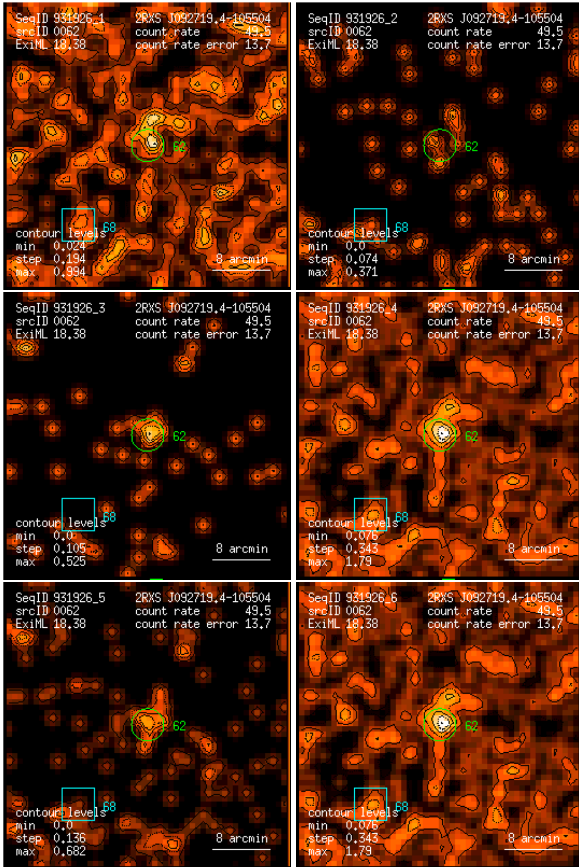
Figure 62: RASS 931926: detection 0062: band rate images, Gaussian filter: (1) PSPC channels 11 – 41, (2) 52 – 90, (3) 91 – 201, (4) 11 – 235, (5) 52 – 201, (6) 11 – 201. Broad band rates in counts/ks. Band rate contour levels in counts/ks/arcmin 2 .
