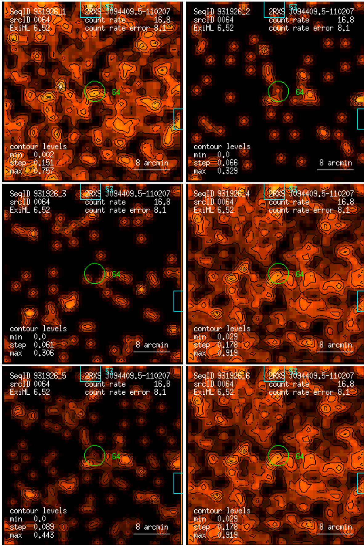
Figure 64: RASS 931926: detection 0064: band rate images, Gaussian filter: (1) PSPC channels 11 – 41, (2) 52 – 90, (3) 91 – 201, (4) 11 – 235, (5) 52 – 201, (6) 11 – 201. Broad band rates in counts/ks. Band rate contour levels in counts/ks/arcmin 2 .
