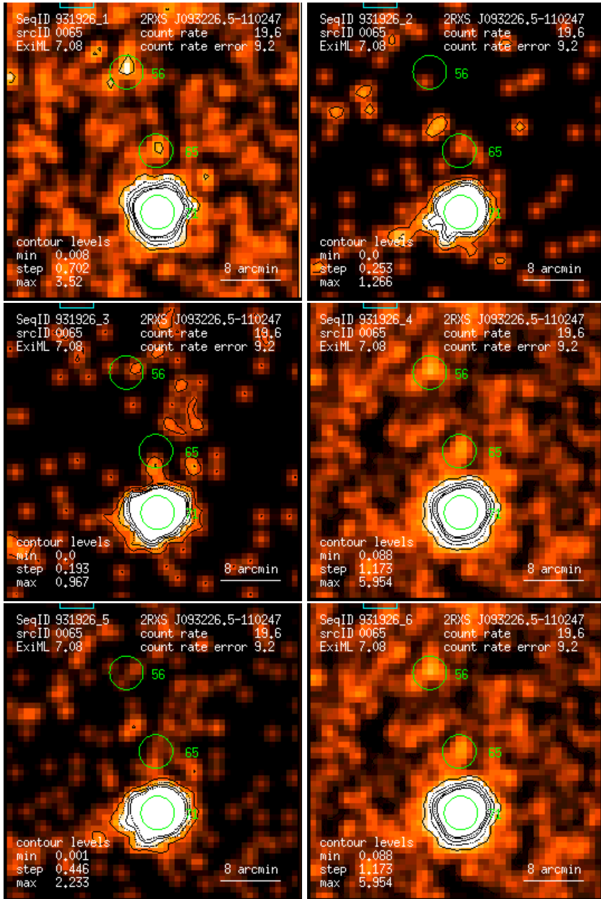
Figure 65: RASS 931926: detection 0065: band rate images, Gaussian filter: (1) PSPC channels 11 – 41, (2) 52 – 90, (3) 91 – 201, (4) 11 – 235, (5) 52 – 201, (6) 11 – 201. Broad band rates in counts/ks. Band rate contour levels in counts/ks/arcmin 2 .
