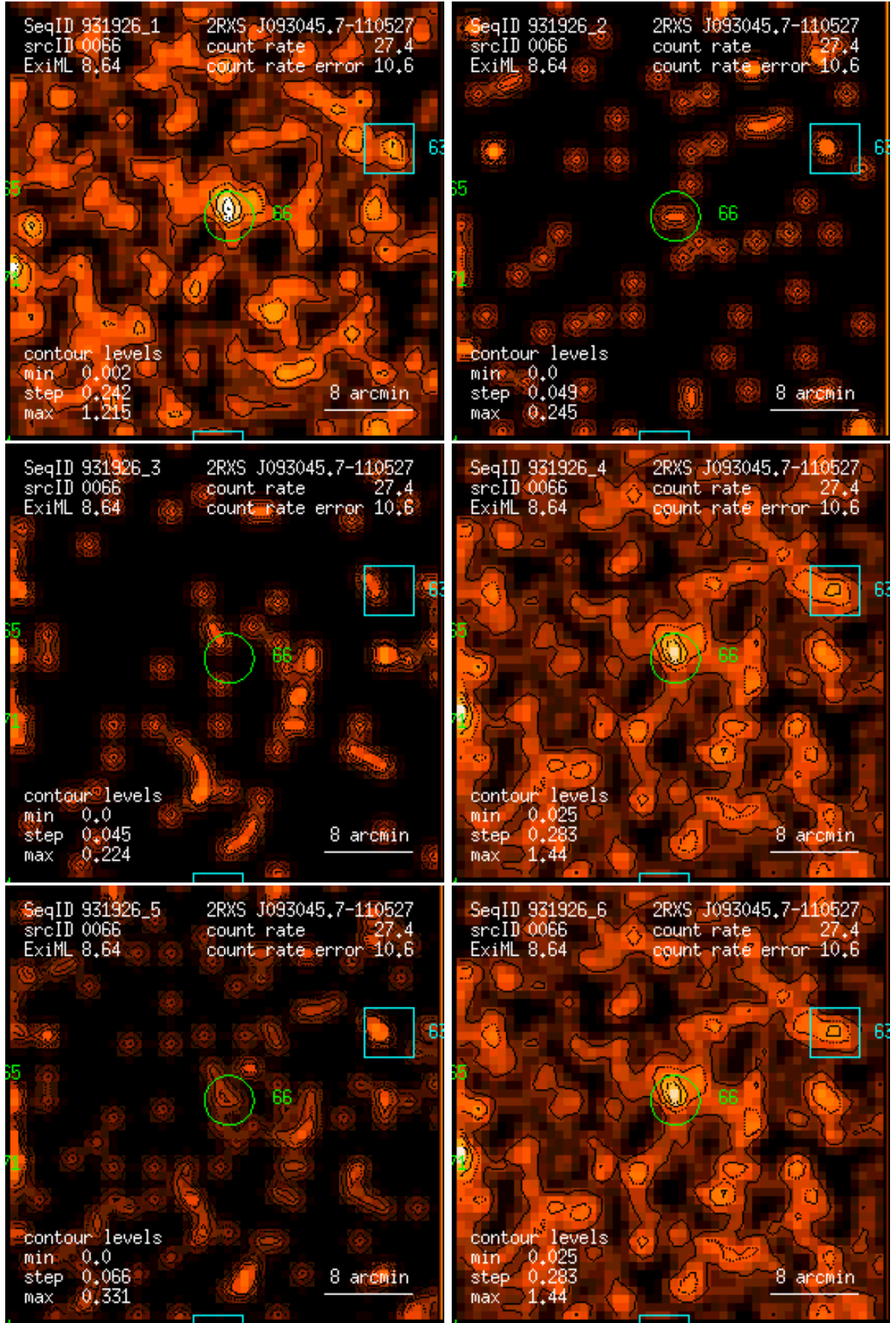
Figure 66: RASS 931926: detection 0066: band rate images, Gaussian filter: (1) PSPC channels 11 – 41, (2) 52 – 90, (3) 91 – 201, (4) 11 – 235, (5) 52 – 201, (6) 11 – 201. Broad band rates in counts/ks. Band rate contour levels in counts/ks/arcmin 2 .
