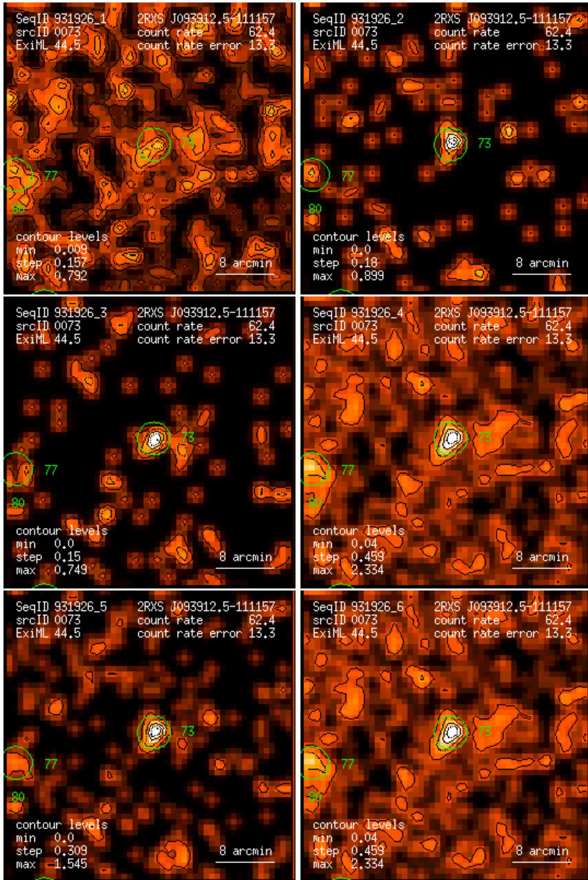
Figure 73: RASS 931926: detection 0073: band rate images, Gaussian filter: (1) PSPC channels 11 – 41, (2) 52 – 90, (3) 91 – 201, (4) 11 – 235, (5) 52 – 201, (6) 11 – 201. Broad band rates in counts/ks. Band rate contour levels in counts/ks/arcmin 2 .
