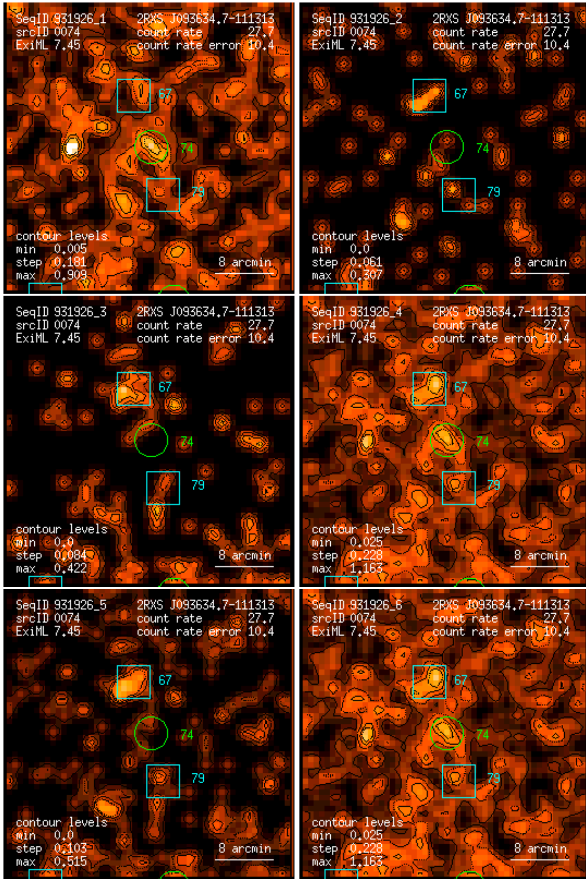
Figure 74: RASS 931926: detection 0074: band rate images, Gaussian filter: (1) PSPC channels 11 – 41, (2) 52 – 90, (3) 91 – 201, (4) 11 – 235, (5) 52 – 201, (6) 11 – 201. Broad band rates in counts/ks. Band rate contour levels in counts/ks/arcmin 2 .
